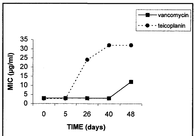
FIGURE 2. Susceptibility to vancomycin and teicoplanin expressed in minimum inhibitory concentrations of Staphylococcus haemolyticus strains for which cultures were obtained on days 0, 5, 26, 40, and 48.
