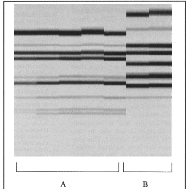
FIGURE 1. Restriction enzyme analysis patterns of five Staphylococcus haemolyticus (A) and two Staphylococcus epidermidis (B) isolates using the staph-PSTI restriction enzyme.
