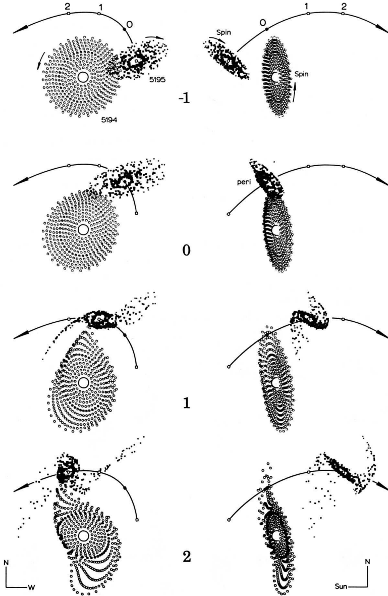
Figure 2. An improved model of the tidal encounter between NGC 5194/5. The left scenes are as if viewed from the Sun, the right set as if from the west. The main revisions from Figure 21 of TT are that the final (= present) time here is only 2.0 instead of 2.4, and that the satellite angles have been changed to i_5 = -75^\circ and \omega_5 = +10^\circ (from -60^\circ , -15^\circ ). Less important, the line of intersection of the 5194 spin plane with the "sky" has been turned to a more realistic PA = -10^\circ , and the main orbit angles have become i_4 = -75^\circ and \omega_4 = -20^\circ . The tilt \beta_4 = -22.5^\circ now. The gravity was also softened moderately at close range.
