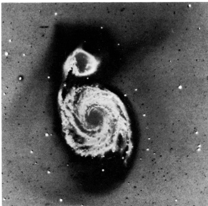
Figure 1. Recent composite photograph of NGC 5194/5, by Burkhead
