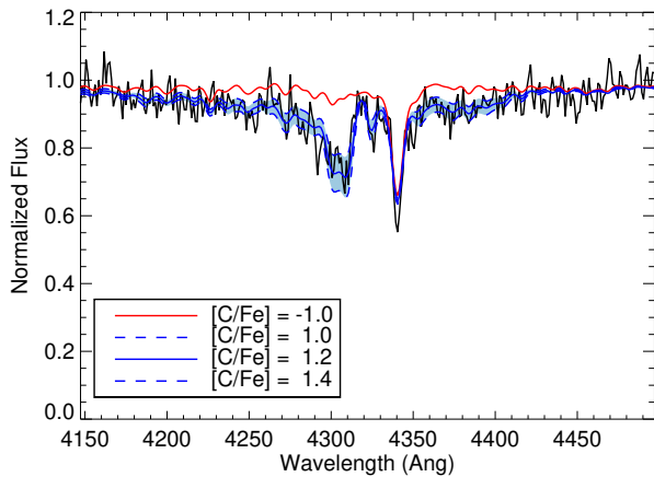
Figure 5. Synthetic spectrum fits to the observed spectrum of star M55 307649. The solid blue line is the best fit ( [C/Fe] = +1.2 ) for the adopted parameters, while the dashed blue lines have [C/Fe] \pm 0.2 about this value. The region between the dashed lines is shaded in light blue to emphasize the regions sensitive to [C/Fe] . The red line shows the synthetic spectrum with the same parameters except that [C/Fe] = -1.0 dex.
