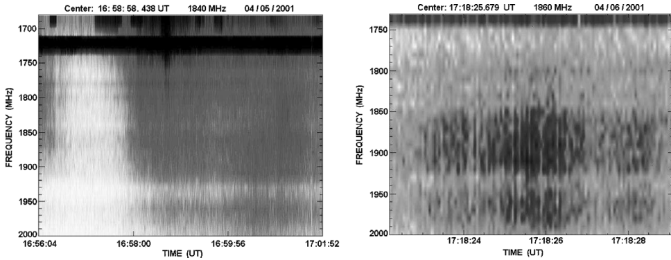
Figure 1. (Left) BSS burst dynamic spectrum associated to CME exhibiting a continuum radio burst emission observed on 04/05/2001 at 16:58 UT. (Right) Pulsation radio emission associated to CME observed on 04/06/2001 at 17:18 UT.
