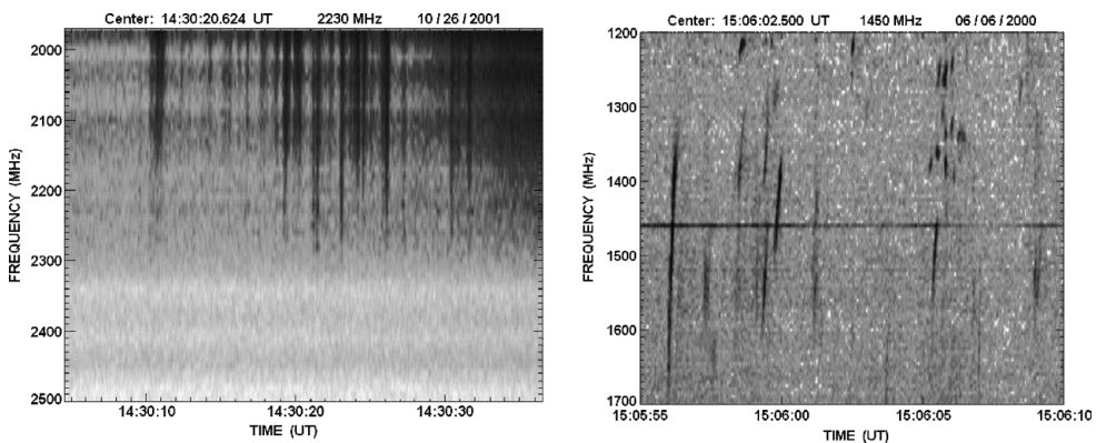
Figure 2. (Left) Dynamic spectrum of BSS bursts observed on 10/26/2001 at 14:30 UT associated to CME. It is clear in the beginning the pulsation emission and its superposition on continuum radio burst emission in the time evolution of the radio burst. (Right) Dynamic spectrum showing a combination of various kinds of radio emission observed by BSS on 06/06/2000 at about 15:06 UT and associated to CME.
