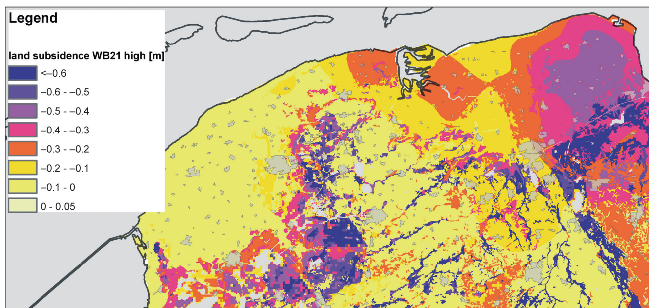
Fig. 3. a. The depth of the brackish-saline interface (1000 mg Cl-/l) in the northern Netherlands. The location of the study areas is shown in the small insert; b. Prognosis of land subsidence in 2100 AD relative to 2000 AD (Haasnoot et al., 1999).
