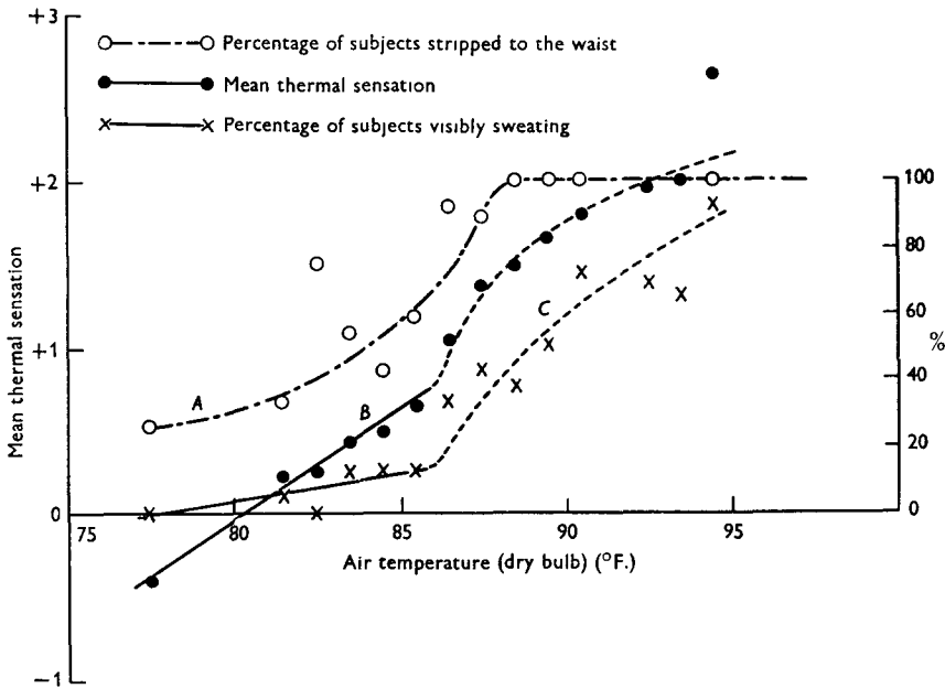
Fig. 3. Mean thermal sensations, percentage of subjects stripped to the waist, and percentage of subjects visibly sweating, related to air temperature (dry bulb) (Ellis, 1952). (Dry bulb range 77–94.9° F. associated with wet-bulb range 70–84.9° F. Effective temperature range 72–85.9° F.).
