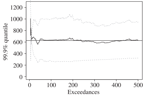
FIGURE 7: Theoretical 99.9% g -and- h quantile (straight solid line) and POT-MLEs for g = 2 and h = 0.2 , based on n = 10^4 observations.
