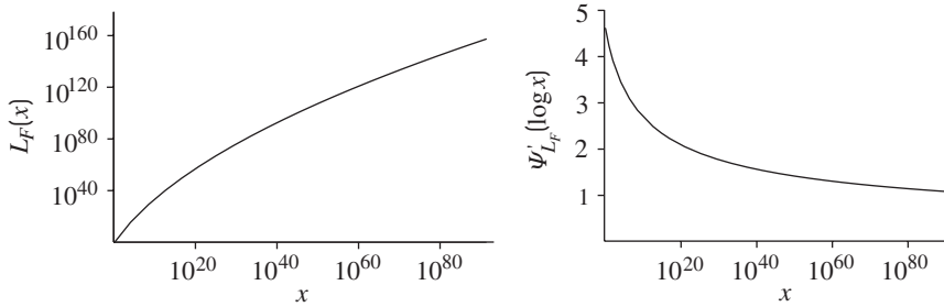
FIGURE 3: Log-log plot of the g -and- h slowly varying function L_F with g = 2 and h = 0.2 (left) with corresponding slope (right) as defined in (4.1).
