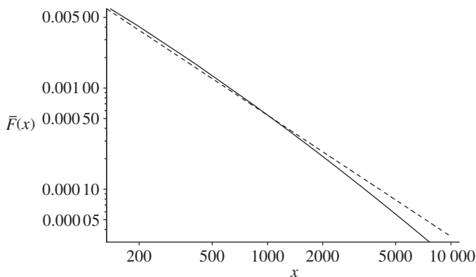
FIGURE 2: Log-log plot of the tail of a g -and- h distribution with g = 2 and h = 0.2 . The straight dashed line l(\cdot) with slope -1.2 is plotted as a reference line.
