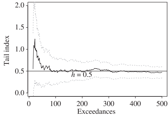
FIGURE 6: Theoretical tail index ( straight solid line ) and POT-MLEs of \xi = h for g -and- h data with g = 0.1 and h = 0.5 , based on n = 10^4 observations.
