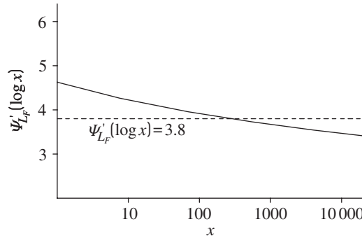
FIGURE 5: Slope of the log-log plot of the g -and- h slowly varying function ( g = 2, h = 0.2 ) in a range relevant for OR.
