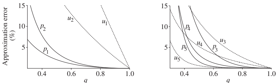
FIGURE 1: Approximation error for the 99.9% quantile of the g -and- h distribution ( g = 2, h = 0.2 ; labels u_1 and p_1 ), the log-gamma distribution ( \alpha = 5, \beta = 5 ; labels u_2 and p_2 ), the Burr distribution ( \alpha = 3, \tau = 1, \kappa = \frac{5}{3} ; labels u_3 and p_3 ), the modified Champernowne distribution ( \alpha = 5, M = 1, c = \frac{1}{4} ; labels u_4 and p_4 ), and the GB2 distribution ( a = 5, b = 1, p = 1, q = 1 ; labels u_5 and p_5 ).
