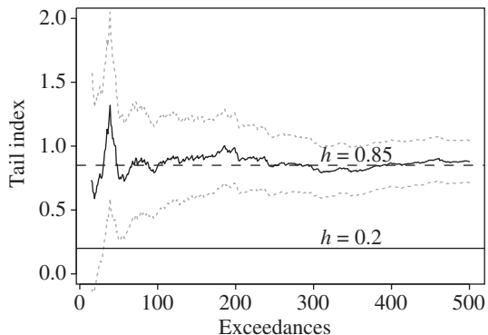
FIGURE 4: Theoretical tail index ( straight solid line ) and POT-MLEs of \xi = h for g -and- h data with g = 2 and h = 0.2 , based on n = 10^4 observations.
