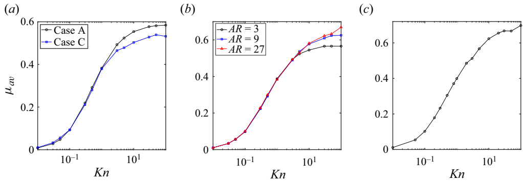
Figure 17. Variations of the width-averaged viscosity \mu_{av}(x=0) (4.4) with Knudsen number: (a) effect of pressure gradient ( \delta p/p_0 = 1 , open black circles; \delta p/p_0 = 0.2 , filled blue circles) on \mu_{av} for AR = 3 (table 3); (b) effect of channel length/aspect-ratio on \mu_{av} for \delta p/p_0 = 0.2 (table 2). (c) Acceleration-driven flow with \hat{a} = 0.1 . For all panels the channel width is L_y/d = 1860 .
