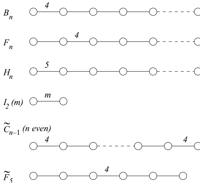
Figure 4. Connected incomplete graphs associated to non simply laced star reducible Coxeter groups.
