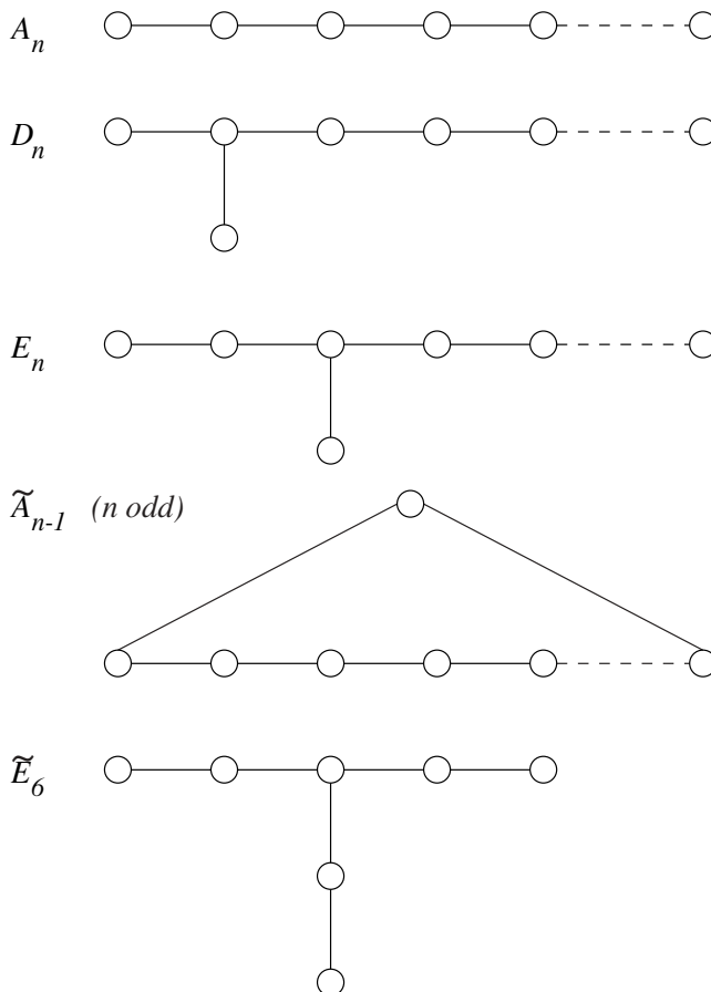
Figure 2. Connected incomplete graphs associated to simply laced star reducible Coxeter groups.
