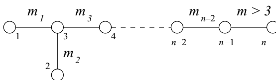
Figure 3. Coxeter graphs considered in the proof of Lemma 6.1.
