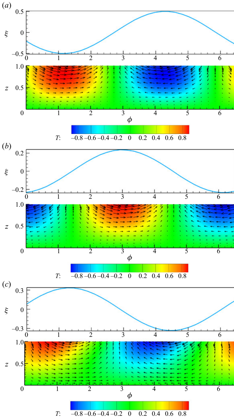
Figure 8. The perturbation flow field and surface deformation at Pr=0.01 , Ca=0.001 and G=100 : (a) Bo=0 , \zeta=0 ; (b) Bo=10 , \zeta=0.5 ; and (c) Bo=0 , \zeta=0.49 . The perturbation phase is defined as \phi = \alpha x + \beta y .
