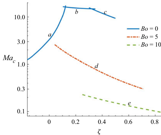
Figure 6. The variation of Ma_c with \zeta and Bo at Pr = 0.01 . The curves correspond to streamwise waves of SWI ( a , c , d and e ) and the oblique wave of CI ( b ).
