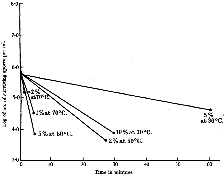
Fig. 2. Rate of death of spores of B. subtilis when submitted to different concentrations of sodium hydroxide at different temperatures.
