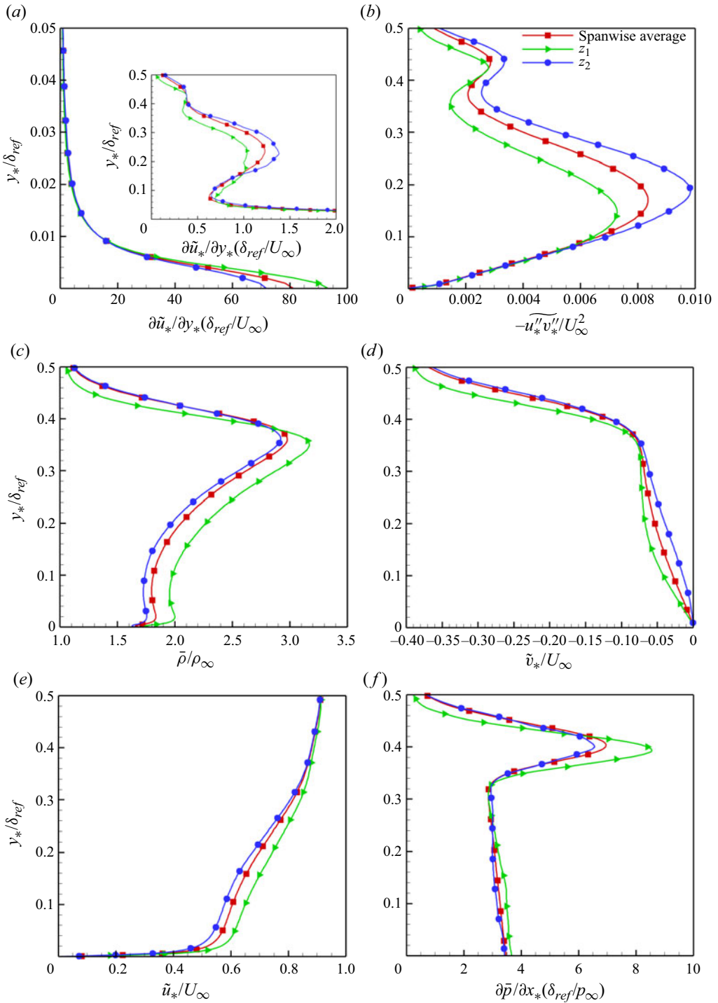
Figure 23. Wall-normal distribution of (a) \partial \tilde{u}_*/\partial y_* , (b) -\tilde{u}_*''\tilde{v}_*''/U_\infty^2 , (c) \bar{\rho} , (d) \tilde{v}_* and \tilde{v}_* , (e) \tilde{u}_* and (f) \partial \bar{p}/\partial x_* at x/\delta_{ref} = 2 for different spanwise positions.
