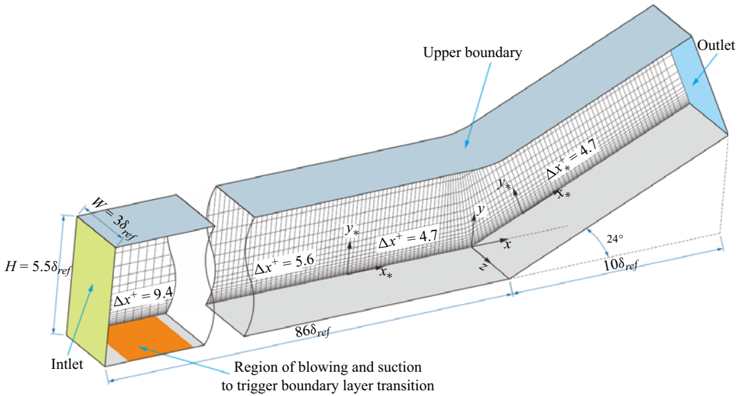
Figure 1. Sketch of the computational domain with its size. Here, \delta_{ref} is the flat-plate turbulent boundary layer thickness at x = -3\delta_{ref} . Mesh distribution in the x - y plane is presented, where the grid point is plotted every 20th grid line in each direction.
