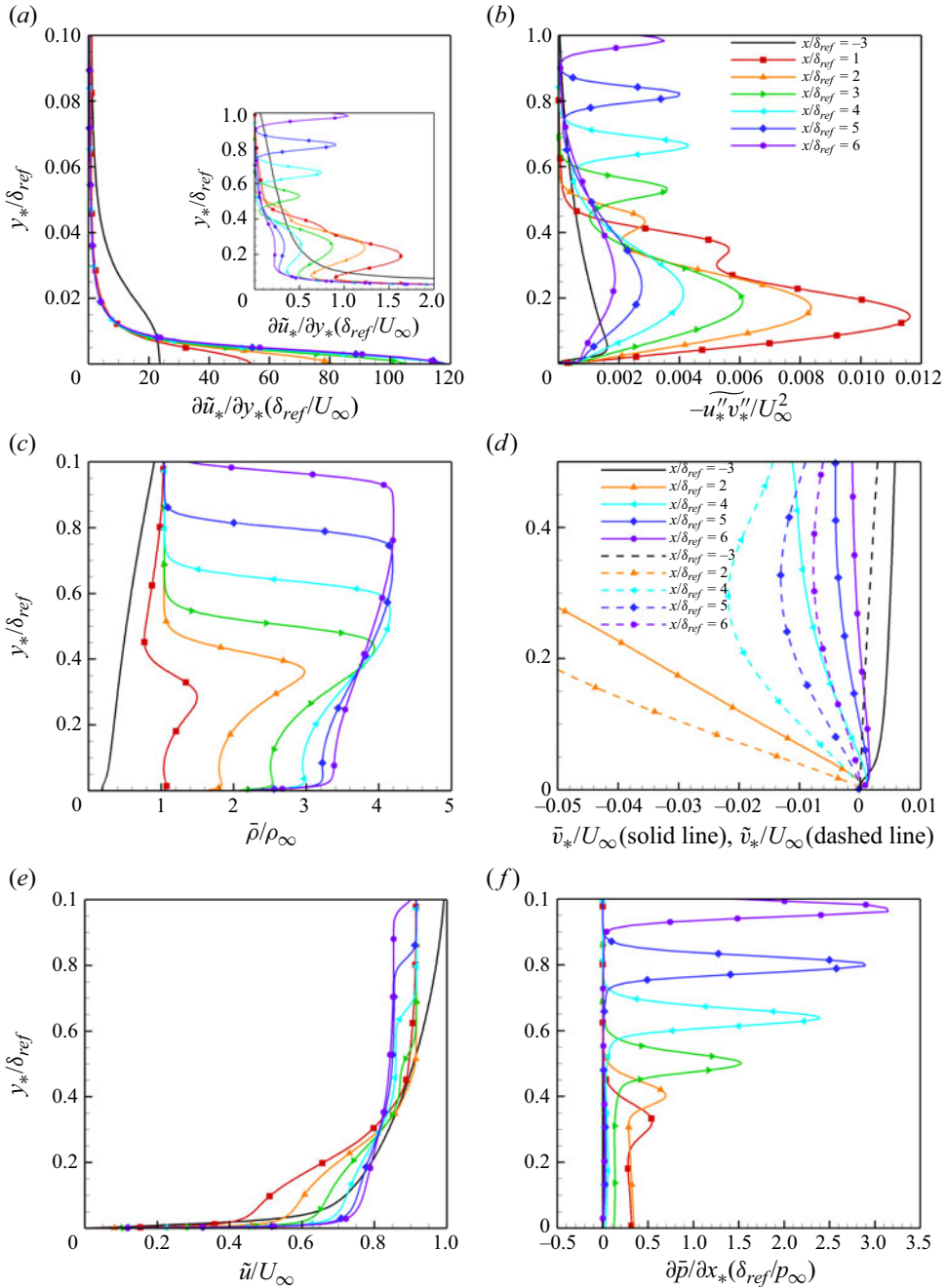
Figure 14. Wall-normal distribution of (a) \partial \tilde{u}_*/\partial y_* , (b) -\tilde{u}''\tilde{v}'' , (c) \bar{\rho} , (d) \tilde{v}_* and \tilde{v}_* , (e) \tilde{u}_* and (f) \partial \bar{p}/\partial x_* at several streamwise locations.
