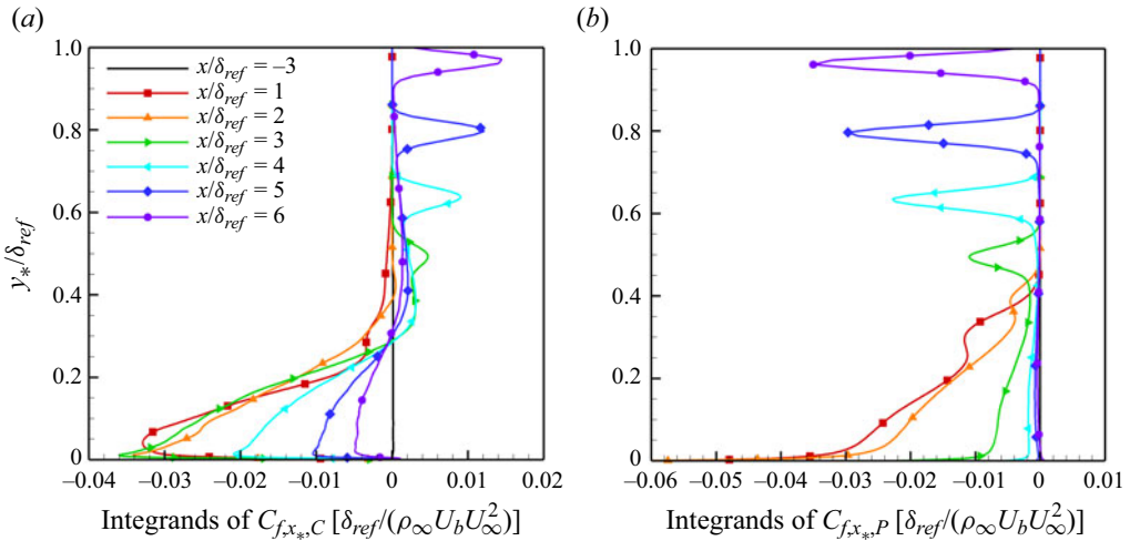
Figure 19. Integrands of (a) C_{f,x^*,C} and (b) C_{f,x^*,P} normalized by \rho_\infty U_b^2 U_\infty / \delta_{ref} at several streamwise locations.
