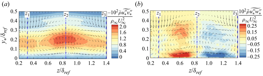
Figure 20. Contours of (a) -\bar{\rho}u''_*\widetilde{v''_* and (b) \bar{\rho}u''_*\widetilde{w''_* in the y_*-z plane at x/\delta_{ref} = 2 . The dashed and dash-dotted lines denote the spanwise stations for maximum and minimum \bar{\tau}_w .
