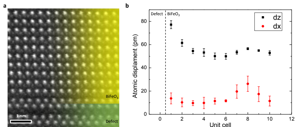
Figure 2. (a) A HADDF STEM image of a polarized BFO region that is in contact with a planar non-stoichiometric defect. (b) Plot of the measured atomic displacements (dz: out-of-plane atomic displacement, dx: in-plane atomic displacement) of Fe cations from the center of four Bi neighbors for BFO atomic structures shown in (a).
