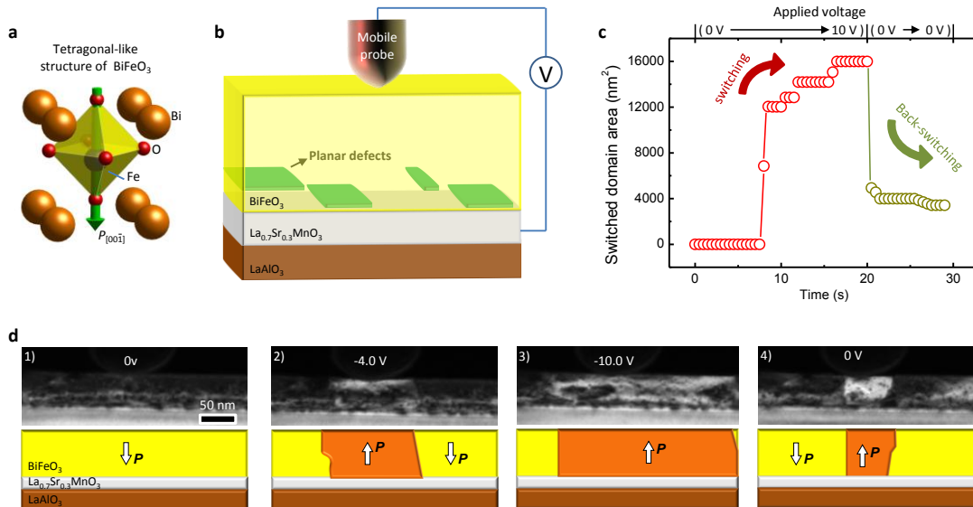
Figure 1. (a) Atomic models of the tetragonal-like structure \text{BiFeO}_3 . (b) Schematic of in situ TEM experimental set-up. (c) Plot of the measured switched domain area versus time extracted from an in situ TEM video. (d) A chronological TEM image series showing the evolution of a written “up” polarized domain in a “down” polarized matrix.
