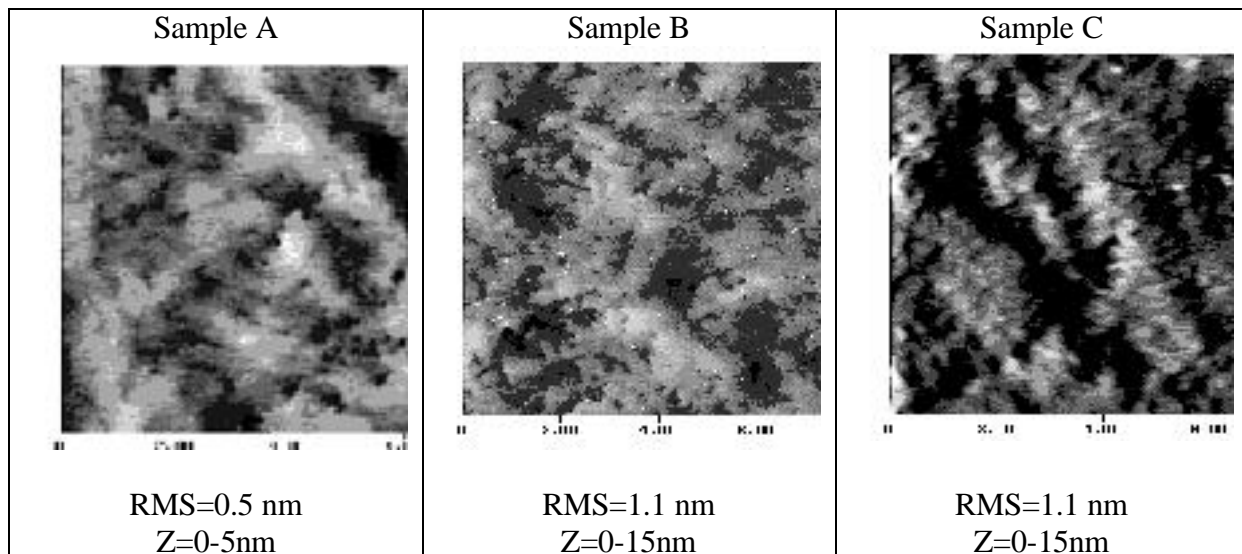
Figure 3: The GaN surface morphology was determined by Atomic Force Microscopy (AFM) for samples grown using DEGaCl or TMGa source. The sample images are obtained over a 10\times 10 micron area. The full range of height (Z) is indicated. The sample structure and related film properties are given in Table 1.
