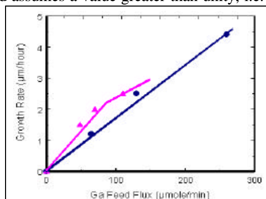
Figure 2. The growth rate of GaN is a function of the calculated Ga flux from the bubbler feed into the reactor for DEGaCl ( - \blacktriangle -) and TMGa ( - \bullet -) sources.
