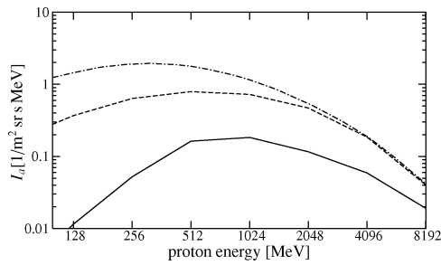
Figure 3. Dash-dotted line: energy spectrum outside the magnetosphere. Dashed line: energy spectrum of cosmic ray protons impacting the atmosphere (100 km above the surface) of an Earth-like exoplanet at 0.2 AU around a 0.5M K/M star. Solid line: energy spectrum of cosmic rays impacting the atmosphere of the Earth. From Griebmeier et al. (2005).
