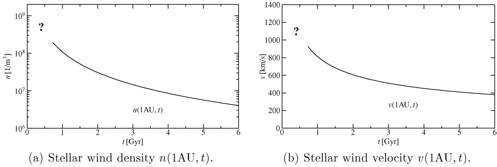
Figure 1. Stellar wind density n(t) and velocity v(t) at 1 AU distance of a sun-like star ( M_{\star} = M_{\odot} , R_{\star} = R_{\odot} ), as a function of stellar age.
