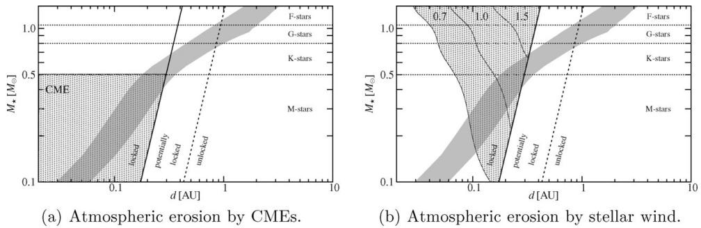
Figure 2. Comparison between the HZ (grey shaded area) and the areas where strong magnetospheric compression is possible by CMEs or stellar wind. The dotted area denotes the region where the magnetosphere can be compressed down to 1.15 Earth radii or less (i.e., 1000 km above the planetary surface). 4.1 Magnetospheric compression by strong CMEs. From Khodachenko et al. (2007). 4.1 Magnetospheric compression by stellar wind of a young star. Three cases are considered: Stellar wind of a star of 0.7 Gyr age (all three dotted areas), Stellar wind of a star of 1.0 Gyr age (upper two dotted areas), Stellar wind of a star of 1.5 Gyr age (top dotted area only).
