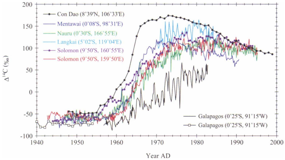
Figure 3 Comparison of a tropical South China Sea coral \Delta^{14}\text{C} record from Con Dao Island (8°39'N, 106°33'E; this study) with coral \Delta^{14}\text{C} records from a latitude range of <math>10^\circ</math>: Mentawai Islands (Grumet et al. 2004), Nauru Island (Guilderson et al. 1998), Langkai Island (Moore et al. 1997), Solomon Islands (Guilderson et al. 2004; Schmidt et al. 2004), and Galapagos Islands (Druffel 1981; Guilderson and Schrag 1998).
