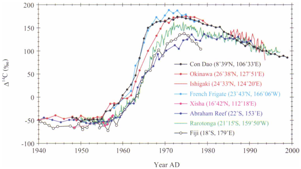
Figure 4 Comparison of a tropical South China Sea coral \Delta^{14}\text{C} record from Con Dao Island (8°39'N, 106°33'E; this study) with coral \Delta^{14}\text{C} records from a latitude range of 16–27°: Okinawa Island (Konishi et al. 1982), Ishigaki Island (Mitsuguchi et al. 2004), French Frigate Shoals (Druffel 1987), Xisha Islands (Southon et al. 2002), Abraham Reef (Druffel and Griffin 1995), Rarotonga Island (Guilderson et al. 2000), and Fiji Islands (Toggweiler et al. 1991).
