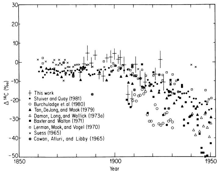
Fig 1. \Delta^{14}\text{C} (uncorrected for the Suess effect)
