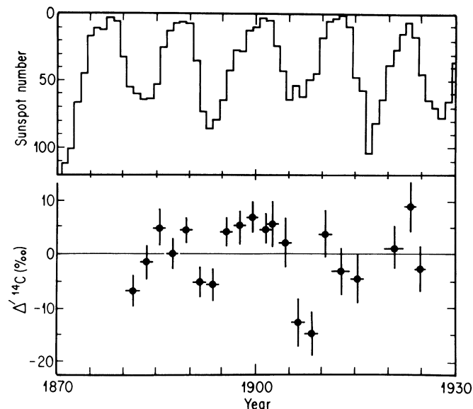
Fig 2. Upper panel: sunspot numbers Lower panel: \Delta'^{14}\text{C} (corrected for the Suess effect)
