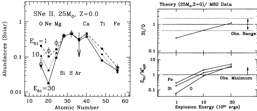
Figure 1. Abundance patterns of M82 compared with hyper(supernova) yields (left). Theoretical models' Si/O mass fraction ratio, and the energy to metal (Fe, Si and O) mass ratios as a function of explosion energy (right).
