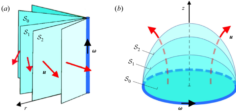
Figure 1. Distinguished isophase surfaces (shades of cyan) \mathcal{S}_0, \mathcal{S}_1, \mathcal{S}_2, \dots associated with (a) a straight vortex, and (b) a vortex ring. The induced velocity field \mathbf{u} is represented by red arrows.
