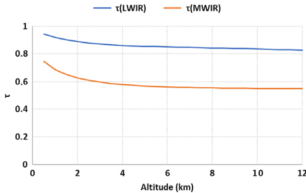
Figure 7. Variation of atmospheric transmission with altitude.
