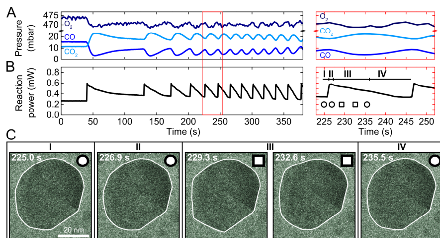
Figure 2. Oscillatory oxidation of CO catalyzed by Pt nanoparticles in the nanoreactor. Simultaneous, time-resolved (A) mass spectrometry of the CO, O 2 and CO 2 pressures, (B) reaction power and (C) HRTEM of a Pt nanoparticle. Reaction conditions: 1.0 bar of CO:O 2 :He at 3%:42%:55% and temperature is 659 K. Adapted from [3].
