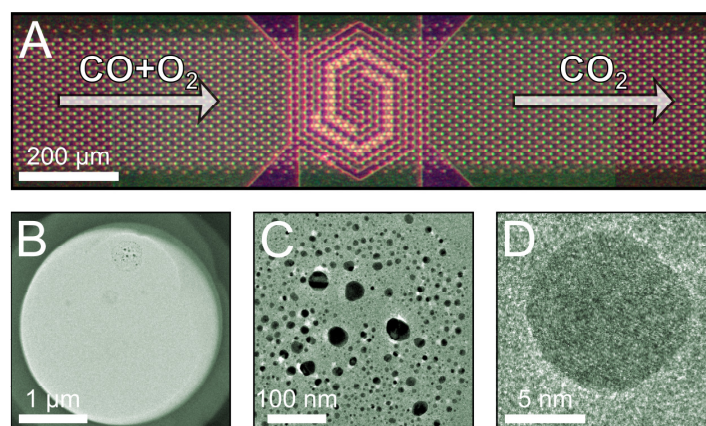
Figure 1. CO oxidation catalyzed by Pt nanoparticles in the nanoreactor. (A) Optical micrograph of the nanoreactor channel with the reaction zone defined by the heater coil and electron-transparent windows for HRTEM. (B-C) Electron micrographs of an electron transparent window and of Pt nanoparticles dispersed on the window. (D) Low dose-rate HRTEM of a Pt nanoparticle in 1 bar CO:O 2 :He = 3:24:55.
