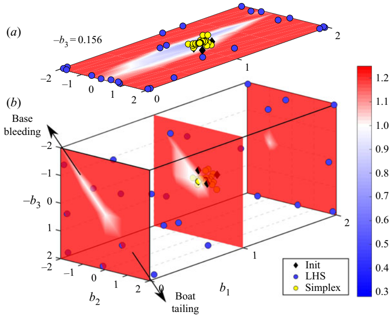
Figure 9. Contour map of J_a/J_0 at the optimal plane b_3 = b^{EGM} = -0.156 found with EGM (a) and at different levels of b_1 : b_1 = 0 , b_1 = 1 , b_1 = 2 (b). The colour code denotes white for J_a/J_0 = 1 , blue for better performances and red for worse performances. The planes are shown with 75 % transparency. The four initial conditions [1, 0, 0]^T , [1.2, 0, 0]^T , [1, 0.4, 0]^T and [0, 0, 0.4]^T are represented by black diamonds. Blue dots are the control laws built with the exploration phases and yellow dots are the individuals built with the exploitation phases. All the individuals have been projected on the plane b_3 = -0.156 . The arrows, on plane b_1 = 0 , depict the base bleeding/boat tailing diagonal studied in § 4.1. A parametric study shows that the minimum is close to [b_1, b_2, b_3]^T = [1, 0, 0]^T whose cost is J_a/J_0 = 0.93 .
