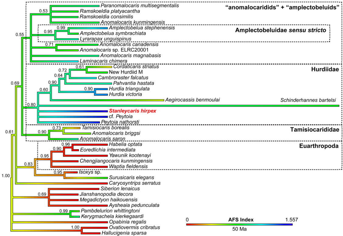
FIGURE 8. Evolution of early panarthropod frontal appendicular functional diversity. Cambrian panarthropod time tree (majority rule consensus), with maximum-likelihood ancestral state reconstruction of Appendicular Functional Specialization (AFS) index for frontal appendages. Numbers at nodes are posterior probabilities.
