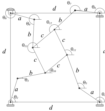
Figure 5. Configurabe parallel manipulator.
