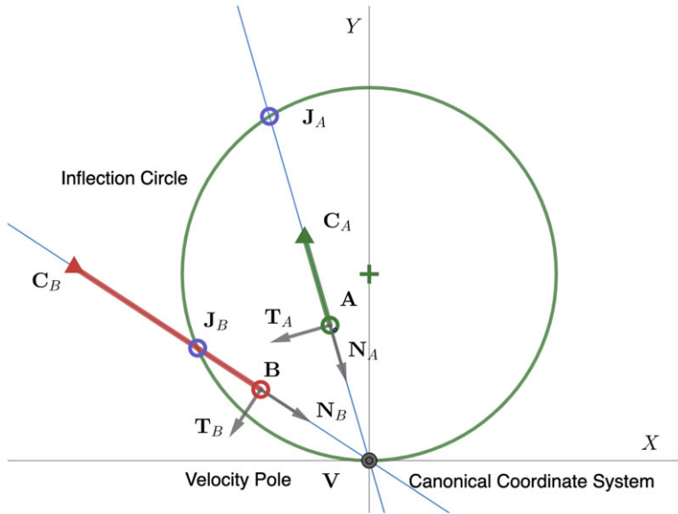
Figure 2. The canonical coordinate system simplifies the equations that define tangent \mathbf{T}_A and normal \mathbf{N}_A vectors for a trajectory \mathbf{A} , as well as for its the center of curvature \mathbf{C}_A .
