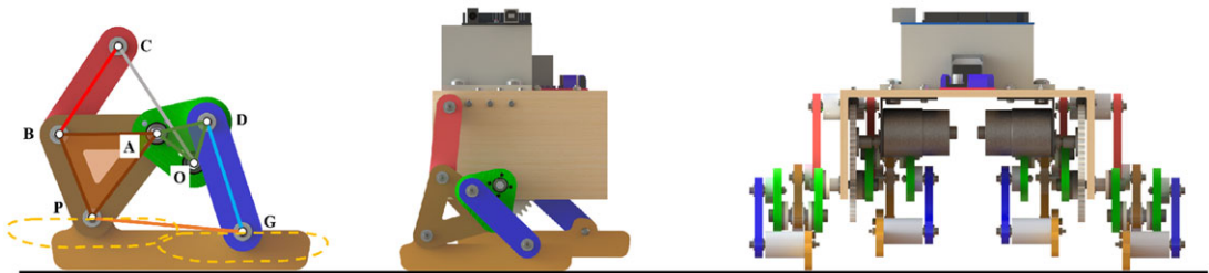
Figure 7. Left: The STAR walker six-bar leg mechanism. Links DG and PG are added to OABC to obtain a non-rotating foot. Center: Two leg mechanisms on one side form a leg system with one actuated input crank. Right: Front view shows the right and left leg systems.
