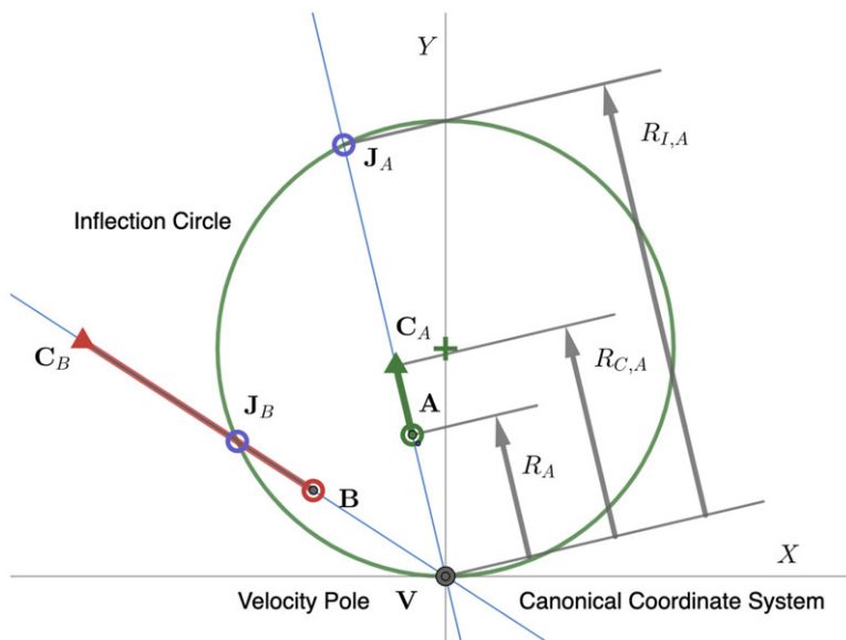
Figure 3. The Euler-Savary equation relates the radial distance to the center of curvature R_{C_A} to the radial distance R_A and the radial distance R_{L_A} to the intersection with the inflection circle.
