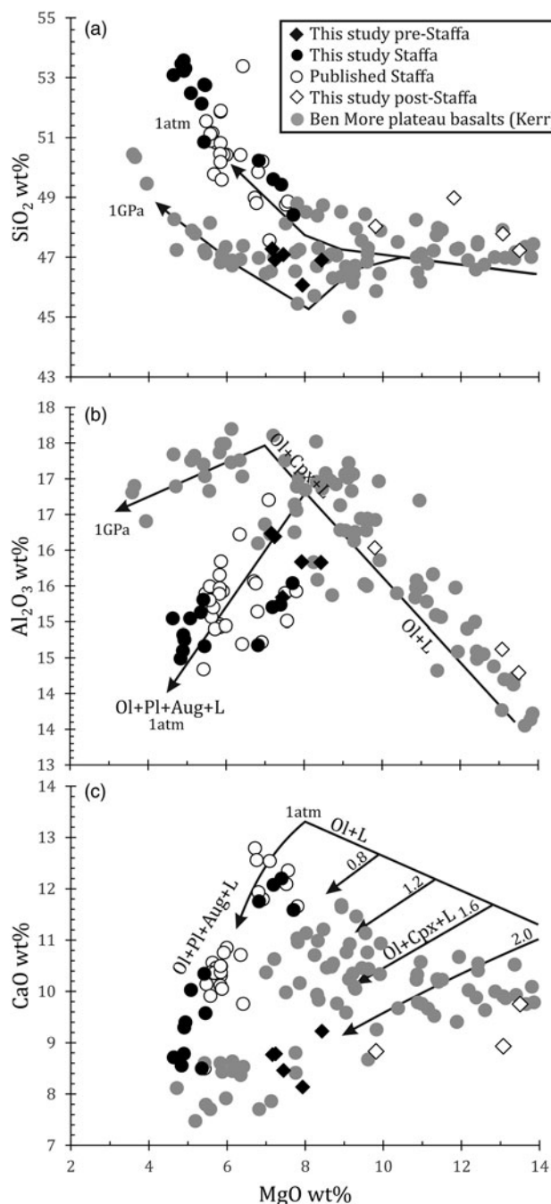
Figure 4 (a) \text{SiO}_2 , (b) \text{Al}_2\text{O}_3 and (c) \text{CaO} versus \text{MgO} (all wt%) for Mull plateau lavas and Staffa-type lava. Mull plateau lavas are represented by the Ben More succession (Kerr et al. 1999) and Staffa lavas are from Thompson et al. (1986), Kerr (1998), Kerr et al. (1999) and Hole et al. (2015). Staffa lava localities are Ardtun Head, Malcolm's Point, Wilderness, Burg and Fingal's Cave (Staffa). Black arrows are schematic LLD taken from Hole (2018). In (a) LLD are shown for \sim 1 GPa and 101.325 kPa and in (b) at variable pressures from 101.325 kPa to 2 GPa as indicated in the figure. Note that at 1 GPa, Cpx (mildly aluminous) joins the liquidus before plagioclase whereas at 101.325 kPa plagioclase joins the liquidus before augite. This results in higher \text{Al}_2\text{O}_3 for lavas with \text{MgO} < 8 wt% that crystallise at 1 GPa compared with those that crystallise at 101.325 kPa. In (b) published Staffa lava data fall close to the predicted 101.325 kPa L + Ol + Pl + Aug cotectic. Abbreviations: LLD = liquid-lines-of-descent; Cpx = clinopyroxene.
