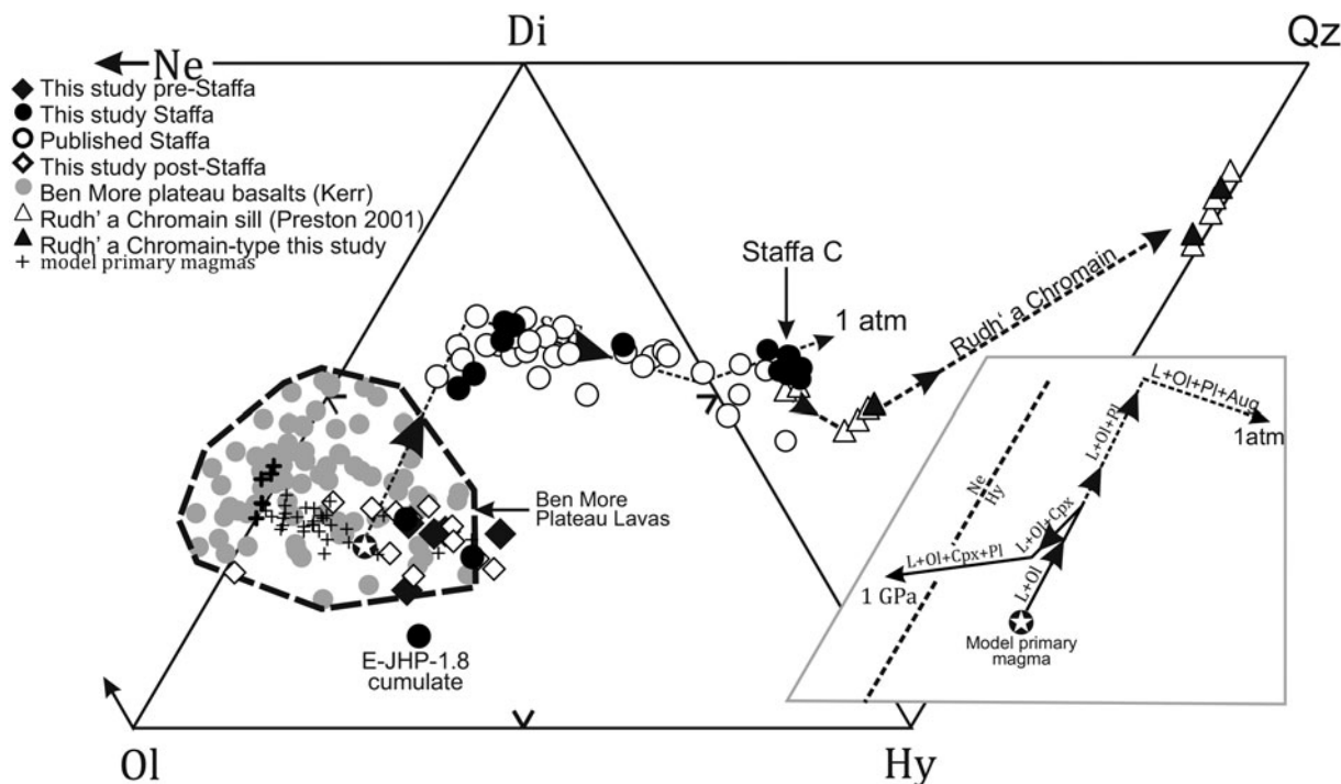
Figure 5 Expanded CIPW normative (wt%) basalt tetrahedron projected from or towards plagioclase onto the planes nepheline-diopside-olivine-hypersthene-quartz (Ne–Ol–Di–Hy–Qz). Data sources as for Fig. 1 except for the Rubha a' Chromain composite sill that is from Preston (2001). Crosses in the Plateau lava data field represent a range of model primary magma compositions for the region (Hole & Millett 2016) with melting decreasing towards and beyond the Ol–Di join. The star in circle is an estimated model primary magma to the Staffa lavas. The inset (right) illustrates the predicted LLDs for a model BPIP primary magma derived from Skye lava SK982 (star in circle; Hole & Millett, 2016) at 101.325 kPa and 1 GPa. These were calculated using Petrolog3 (Danyushevsky & Plechov 2011) using the Ol model of Beattie et al. (1991) and plagioclase and augite models of Danyushevsky (2001). The QFM buffer was that of Kress & Charnick (1988) and QFM-1 was assumed. Note that at 1 GPa, Cpx (aluminous) joins the liquidus before plagioclase such that the LLD moves towards more Si-undersaturated compositions with decreasing MgO and may ultimately cross the Ol–Di join. At 101.325 kPa, plagioclase joins the liquidus before augite and the LLD projects towards the Di axis; thereafter, crystallisation along the L + Ol + Pl + Aug cotectic results in final liquids occupying an area in the Di–Hy–Qz field of the diagram. Staffa lavas follow the 101.325 kPa LLD whereas, typically, plateau basalts follow the 1 GPa LLD (Thompson 1982; Hole et al. 2015; Hole 2018). Abbreviations: CIPW = Cross, Iddings, Pirsson and Washington norm; LLD = liquid-lines-of-descent; BPIP = British Palaeogene Igneous Province; QFM = quartz–fayalite–magnetite; Cpx = clinopyroxene.
