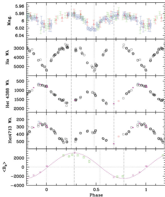
Figure 2. Phased observational data: Photometric data from Oksala et al. (2010), and ASAS data from Mikulášek et al. (2010) (uppermost), EWs from UVES (middle), with FORS and FEROS W_\lambda measurements of HeI 4388, 4713 added, as well as FORS (Rivinius et al. (2010)) and ESPaDOns magnetic data (lowermost panel).
