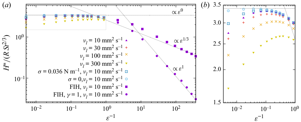
Figure 3. (a) Plot of rescaled initial stagnation height H^*/(RSt^{2/3}) as a function of the inverse of the dimensionless compressibility parameter \epsilon = P_0RSt^{4/3}/\mu_g V , for a range of different liquid viscosities \nu_l , surface tensions \sigma and gas parameters \gamma . Unless otherwise stated, baseline parameters from tables 2 and 3 are used. By default, the drop starts from a height H_0 scaled according to (2.13). For \nu_l = 10 \text{ mm}^2 \text{ s}^{-1} , to account for compressibility effects, data from two simulation sequences that use a fixed initial height (FIH) based on substituting V = 2 \text{ m s}^{-1} into (2.13) are shown. (b) Zoomed-in plot of the same data, showing the region bounded by the dotted grey rectangle in panel (a).
