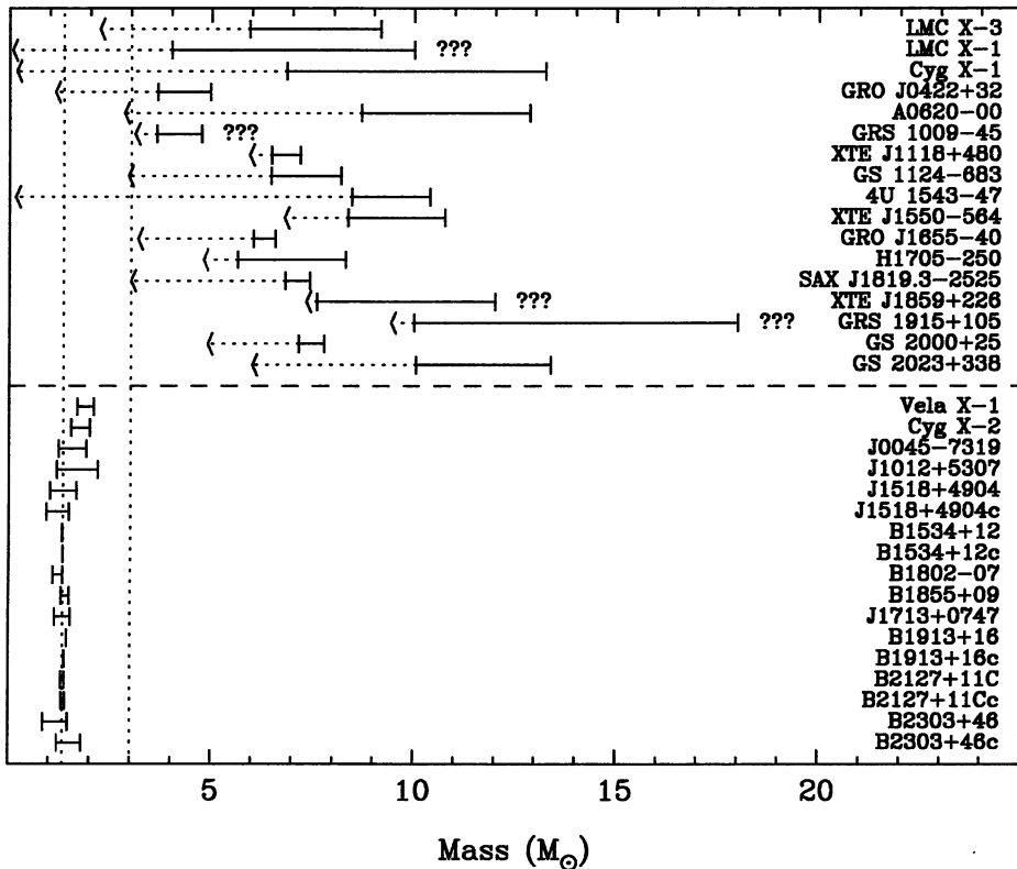
Figure 1. Black hole masses ( top , Table 1 and cited references) and selected neutron star masses ( bottom , Thorsett & Chakrabarty 1999). Ranges are 1\sigma in most cases. Arrows in the top indicate measured mass functions.
