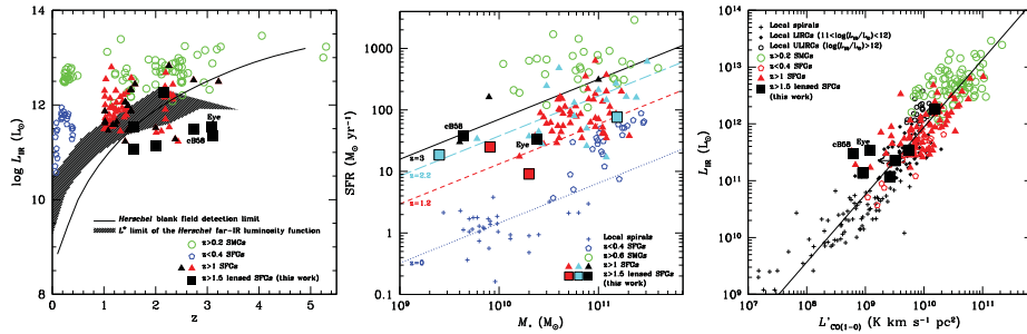
Figure 1. Comparison of the lensed, sub- L^* SFGs with our compilation of CO-detected galaxies from the literature (see Dessauges-Zavadsky et al. 2015). IR luminosities as a function of redshift ( left ), star formation rates as a function of stellar masses with the color-coding referring to 3 redshift bins ( middle ), and IR luminosities as a function of CO(1–0) luminosities ( right ).
