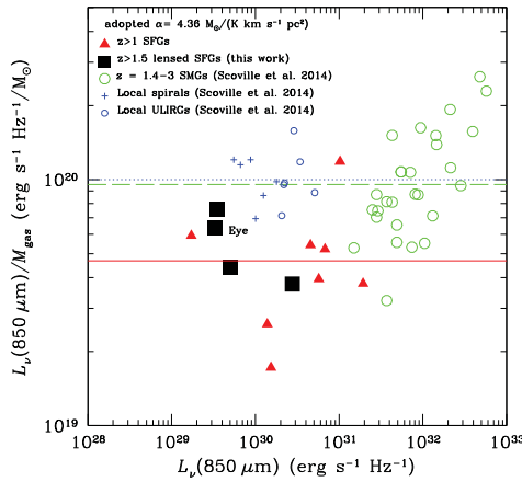
Figure 3. Dust-to-gas ratios estimated from the 850 \mu\text{m} continuum over the molecular gas mass ratio following Scoville et al. (2014) prescriptions. Local spirals, local ULIRGs, high-redshift sub-mm galaxies, and high-redshift SFGs at fixed about solar metallicity are compared.
