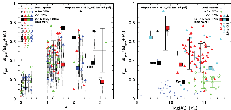
Figure 2. Left: Molecular gas fractions as a function of redshift with the color-coding referring to 4 M_* bins. A net f_{\text{gas}} rise is observed from z = 0 to z \sim 1.6 . Right: Molecular gas fractions as a function of stellar masses with the color-coding referring to 3 redshift bins. A clear f_{\text{gas}} upturn is found at the low- M_* end.
