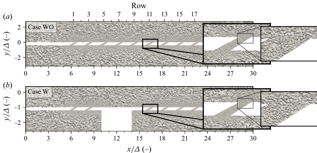
Figure 4. Crinkle view of the mesh on the centreplane \mathcal{P}_{xy,0} of the set-up for case WO (a) and case W (b), along with a zoom on the mesh of perforation H108.
