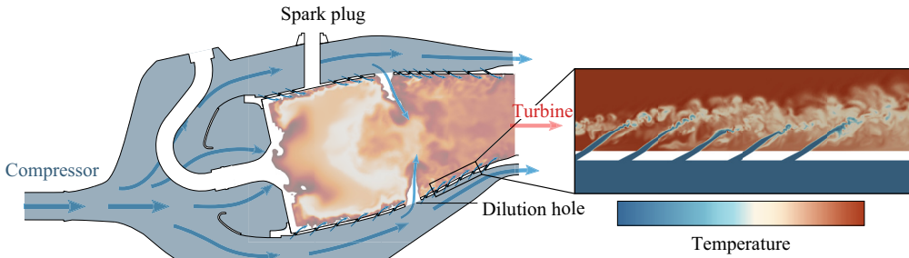
Figure 1. Principle of effusion cooling by multiperforation.
