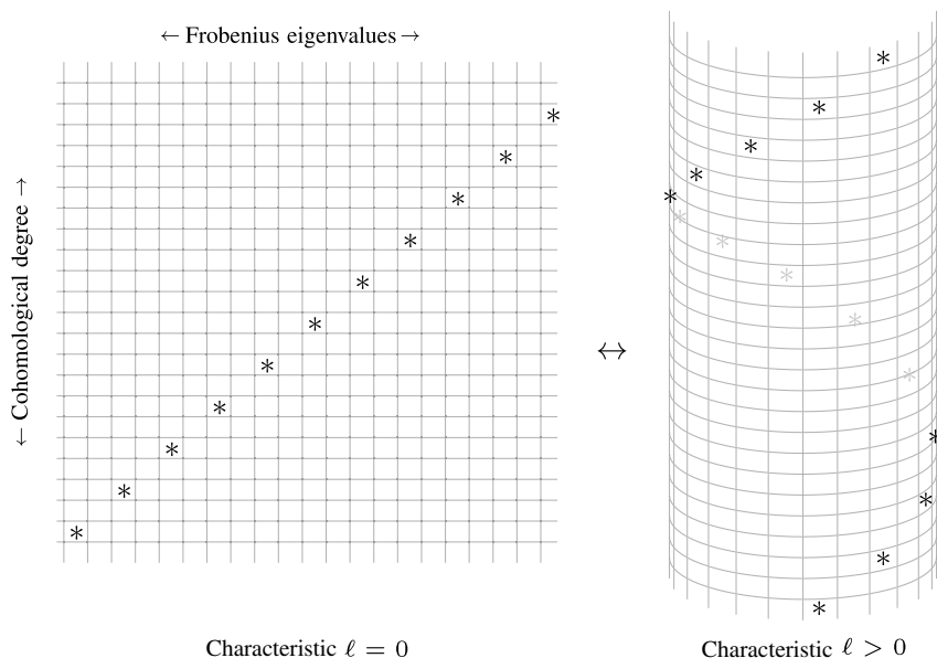
FIGURE 1. Picture of the ‘bigrading’ on E^\bullet (the stars indicate possible non-zero terms in E = H^\bullet(E^\bullet) ).
