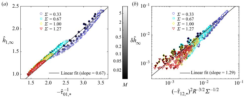
Figure 6. Comparison of the asymptotic thicknesses \hat{h}_{1,\infty} and \delta \hat{h}_\infty obtained numerically with the predictions of scaling laws derived from the virtual contact point model for (a) the lower film (3.2) and (b) the upper film (3.6). The solid lines are best linear fits, yielding prefactors 0.67 and 1.29 for the lower and upper films, respectively. The data presented correspond to various values of \Sigma (symbol shape), M (greyscale) and \Delta H (not marked).
