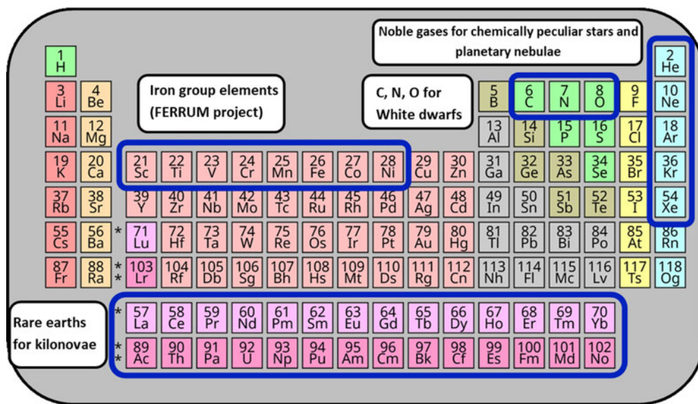
Figure 1. Examples of atomic data needs for different astronomical objects.
