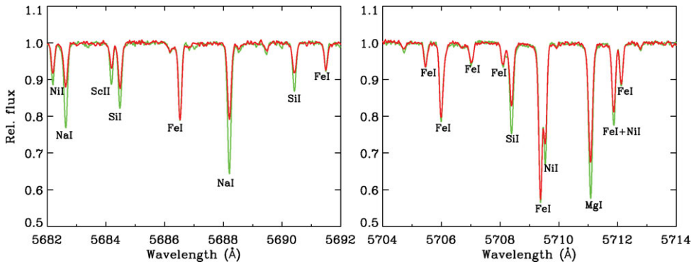
Figure 3. Spectra of two stars with nearly the same atmospheric parameters T_{\text{eff}} , \log g and [\text{Fe}/\text{H}] . The spectrum of the “low- \alpha ” star CD -45 3283 ( T_{\text{eff}} = 5603 K, \log g = 4.57 , [\text{Fe}/\text{H}] = -0.89 , [\alpha/\text{Fe}] = 0.08 ) is shown with a thick (red) line, and that of the “high- \alpha ” star G 159-50 ( T_{\text{eff}} = 5648 K, \log g = 4.39 , [\text{Fe}/\text{H}] = -0.92 , [\alpha/\text{Fe}] = 0.29 ) with a lighter (green) line.
