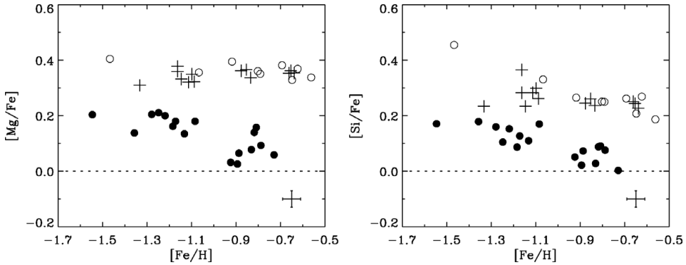
Figure 1. [\text{Mg}/\text{Fe}] and [\text{Si}/\text{Fe}] vs. [\text{Fe}/\text{H}] for the sample of stars with VLT/UVES spectra. Crosses: Thick-disk stars; Open circles: “High- \alpha ” halo stars; Filled circles: “Low- \alpha ” halo stars. Typical error bars for the data are shown in the lower right corners of the figures.
