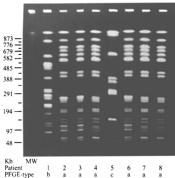
Fig. 3. Analysis of Spe I restriction endonuclease-digested genomic DNA of B. cepacia by pulsed-field gel electrophoresis. Strains isolated from the sputum of case-patients (patients 2–4, 6–8) had an identical RFLP pattern (designated ‘a’ that differed substantially from that of strains from cystic fibrosis patients with B. cepacia respiratory colonization (patients 1 and 5; RFLP patterns ‘b’ and ‘c’). Bacteriophage \lambda ladder (lane MW) was used as molecular size standard. The results were confirmed using Xba I restriction endonuclease digestion.
