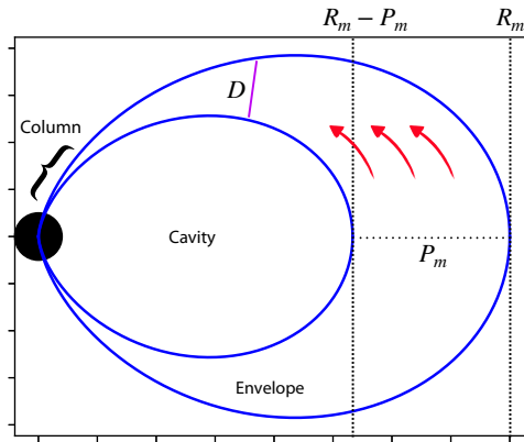
Figure 1. A cartoon of the model set-up of the optically thick envelope. Two bounding magnetospheric field lines are shown in blue. The larger and smaller arcs show dipole field lines reaching out to radii R_m and R_m - P_m respectively. The purple line shows an example, for a particular latitude, of the shortest path along which the radiation diffuses outward and is labelled by the distance D . The black circle represents the surface of the NS. The red arrows show the accretion flow.
