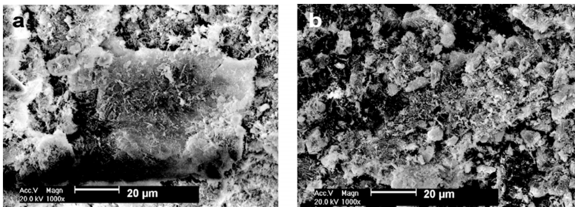
Figure 5. ESEM images of the kaolin sample before (a) and after (b) bioleaching treatment.
