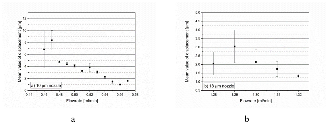
Figure 4. The mean value of displacement as a function of the flowrate for orifice sizes of 10 \mu\text{m} (a) and 18 \mu\text{m} (b). The error bar represents the standard deviation of three independent measurements.
