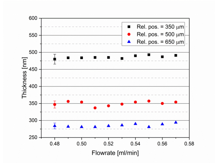
Figure 9. Thickness of the liquid leaf at a certain point on the vertical symmetry axis as a function of the flowrate (10 \mu\text{m} orifice size).
