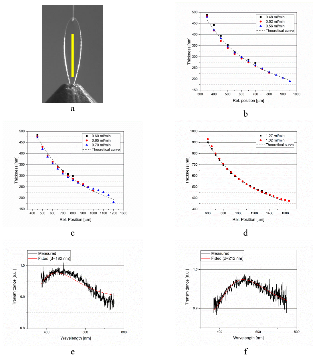
Figure 8. The thickness variation along the vertical axis (a) of the liquid leaf at different flowrates of water (orifice size: b) 10 \mu\text{m} c) 11 \mu\text{m} and d) 18 \mu\text{m} ). The measured and evaluated spectral interference fringe is shown for the two thinnest values of 182 nm (e) and 212 nm (f). The error of the measurement was 3%.
