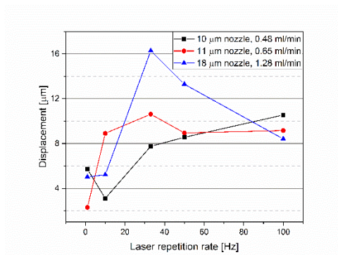
Figure 5. Displacement of the liquid sheet generated by periodic laser pulses for various orifice sizes as a function of the laser's repetition rate. (The lines are only to guide the eye.)
