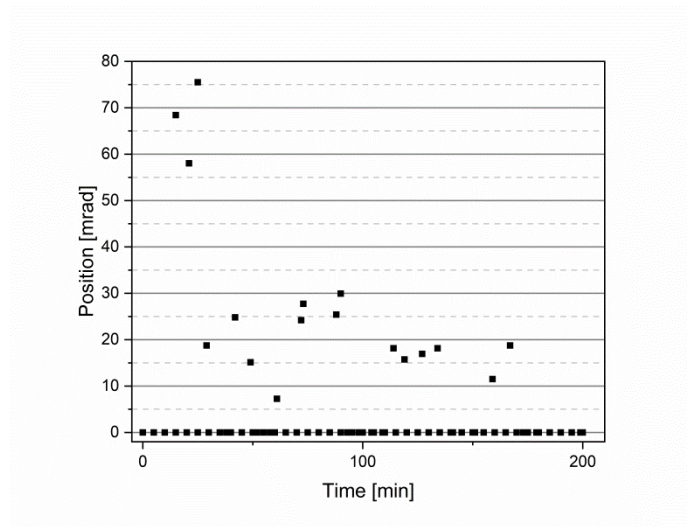
Figure 13. Endurance test results of the continuously working liquid jet. The data show the required rollback angle to the original direction of the liquid leaf, using the reflected light during the experiment.
