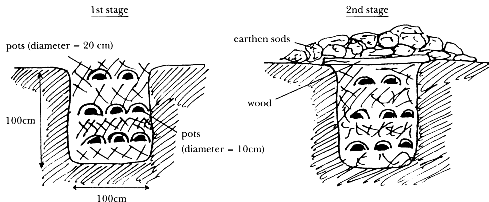
Fig 2. Construction of reducing kilns
