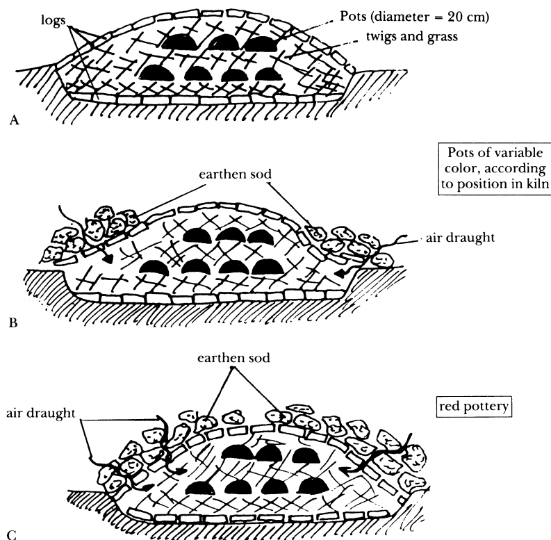
Fig 1. Construction of oxidizing kilns—A and B mildly oxidizing, C highly oxidizing
