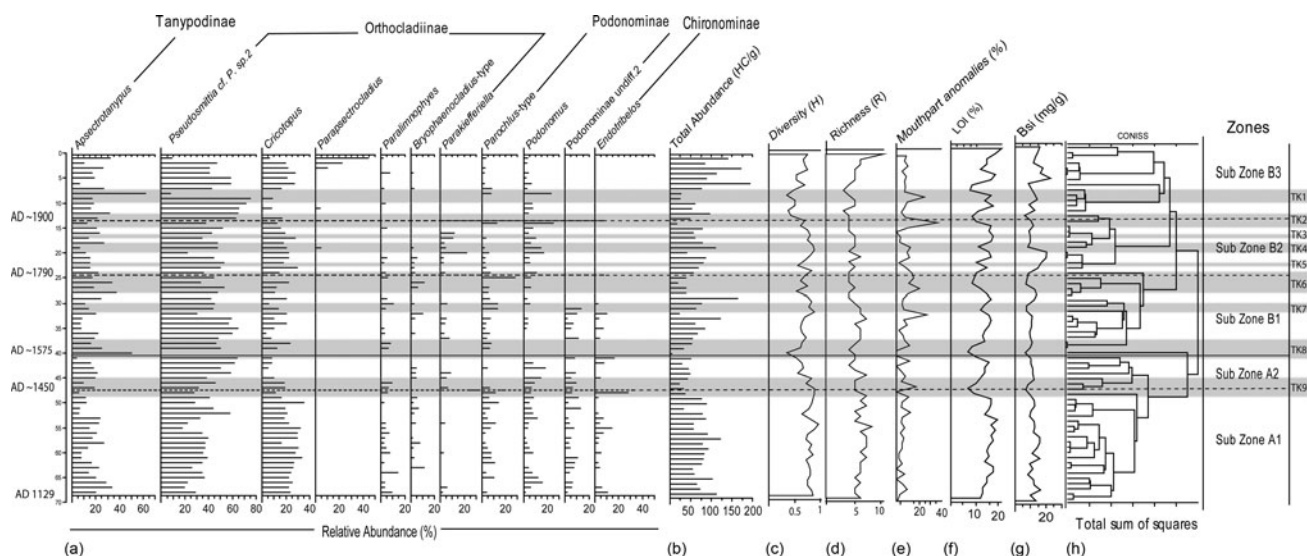
Figure 4. (a) Relative abundance of Chironomidae taxa of Lake Tonček; (b) total abundance of head capsules (HC/g); (c) diversity index (H); (d) richness (R); (e) mouthpart anomalies (%); (f) loss on ignition (LOI, %); (g) biogenic silica (BSI) concentration profile (mg/g); (h) chironomid zones calculated by a CONISS cluster analysis (Tilia version 1.7.16). Volcanic ash layers are presented in gray (TK1–TK9).
