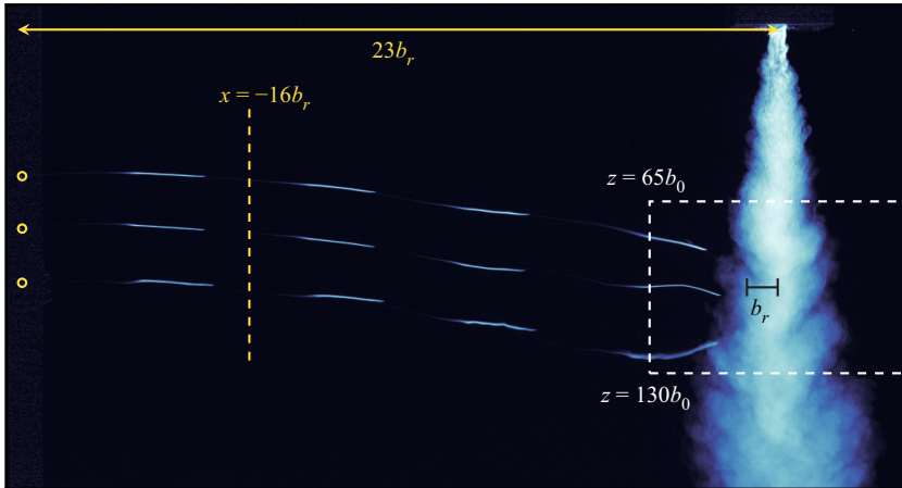
Figure 6. Instantaneous image of a saline plume and its induced-flow field. The entrainment coefficient was determined from combined measurements of: (i) the average velocity of dyline segments for x \in [-16b_r, 5b_r] (approximately) and (ii) the plume scalar width in the region bounded by the dashed white outline. The representative length scale b_r is the plume half-width evaluated at the midpoint of the measurement region ( z = 97.5b_0 ). Circles at x = -23b_r indicate the sources of the dylines.
