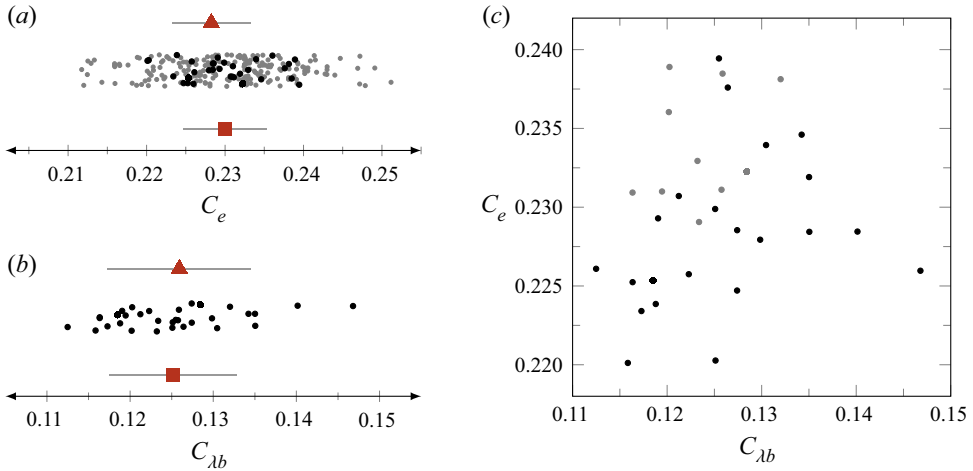
Figure 9. (a) Values of C_e . (b) Values of C_{lb} . In (a), in grey, values for every individual dyeline segment ( 6 \times 32 dots). In (a,b), \bullet average value for each of the 32 experiments; \blacktriangle average value and standard deviation across the centred dyeline experiments; \blacksquare average value and standard deviation across all 32 experiments. (c) Value of C_e against C_{lb} for each of the 32 experiments, grey dots denote an off-centred dyeline experiment; the scatter indicates there is no clear correlation between the two quantities (Pearson’s correlation coefficient of 0.19. The p -value is 0.29 so the null hypothesis of no correlation is not rejected at the 5% significance level).
