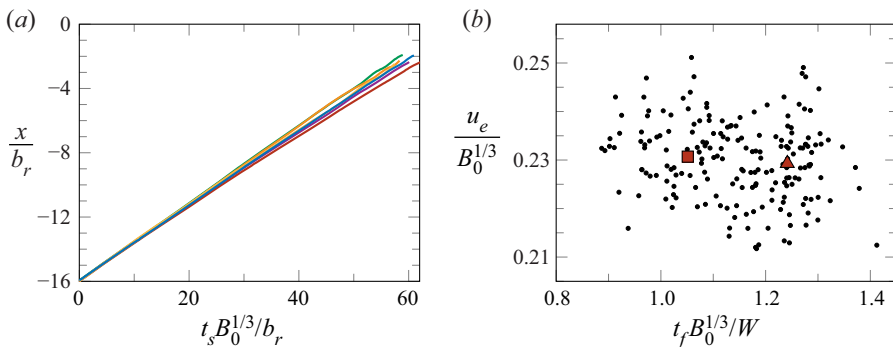
Figure 7. (a) Dimensionless position x/b_r of the leading edge of six dyline segments against time t_s B_0^{1/3}/b_r from Exp. 17. The time origin t_s = 0 was taken as the first frame where the leading edge of a segment crossed the ‘start’ line at x/b_r = -16 . (b) Entrainment velocity u_e/B_0^{1/3} against measurement time t_f B_0^{1/3}/W , where W (= 2770 \text{ mm}) is the tank width, for all 192 segments measured to determine C_e (Pearson’s correlation coefficient of -0.18 ). The p -value is 0.01 and the null hypothesis of no correlation is rejected at the 5% significance level). Ensemble average velocity and measurement time for the first (■) and second (▲) waves of 96 segments.
