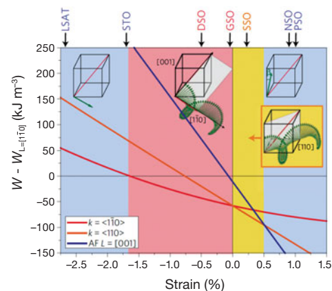
Proposed magnetic phase diagram for BiFeO 3 as a function of strain state. For strains ranging from -1.6% to 0.5%, a Type-I (red) spin cycloid with wave vector along [1\bar{1}0] or a Type-II (orange) spin cycloid with average wave vector along [110] is preferred. However, at higher strains a collinear antiferromagnetic ordering (blue) is preferred. Reproduced with permission from Nature Mater. (2013), DOI: 10.1038/nmat.3629. © 2013 Macmillan Publishers Ltd.
