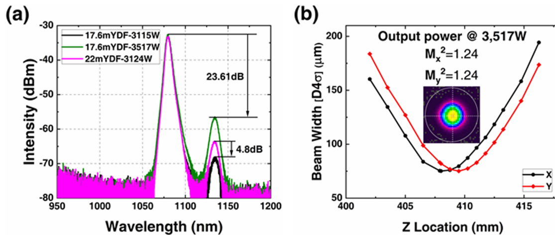
Figure 5. Experimental results of bidirectional pumping after shortening the active fiber of the amplifying section: (a) spectral comparison before and after the shortening of the fiber; (b) result of the beam quality M^2 factor at the power of 3517 W. Inset: a beam profile of the output laser.
