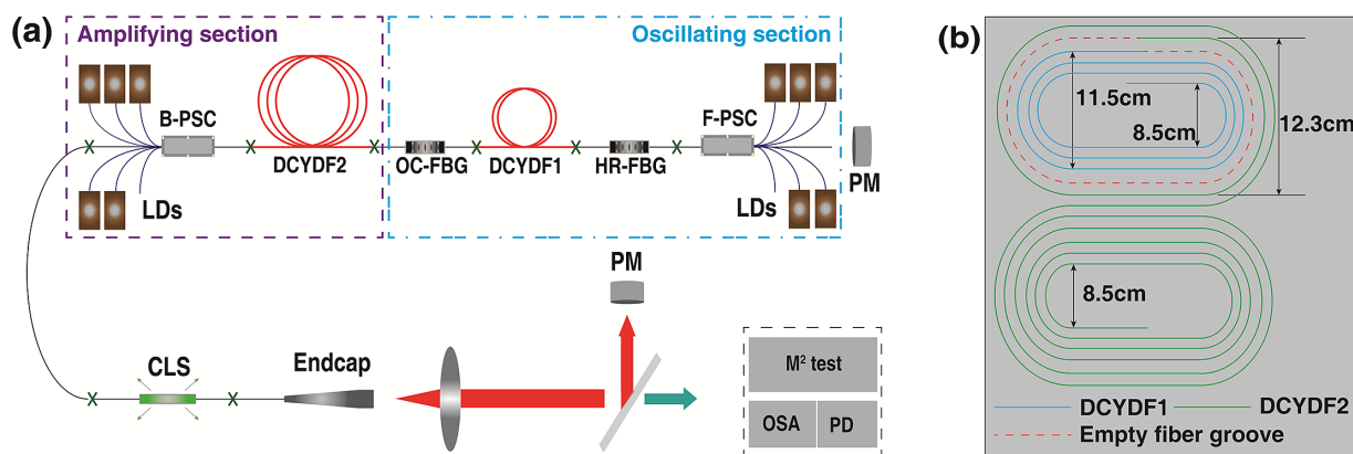
Figure 2. Schematic of the bidirectionally pumped OAILF: (a) experimental structure; (b) schematic diagram of the fiber groove.
