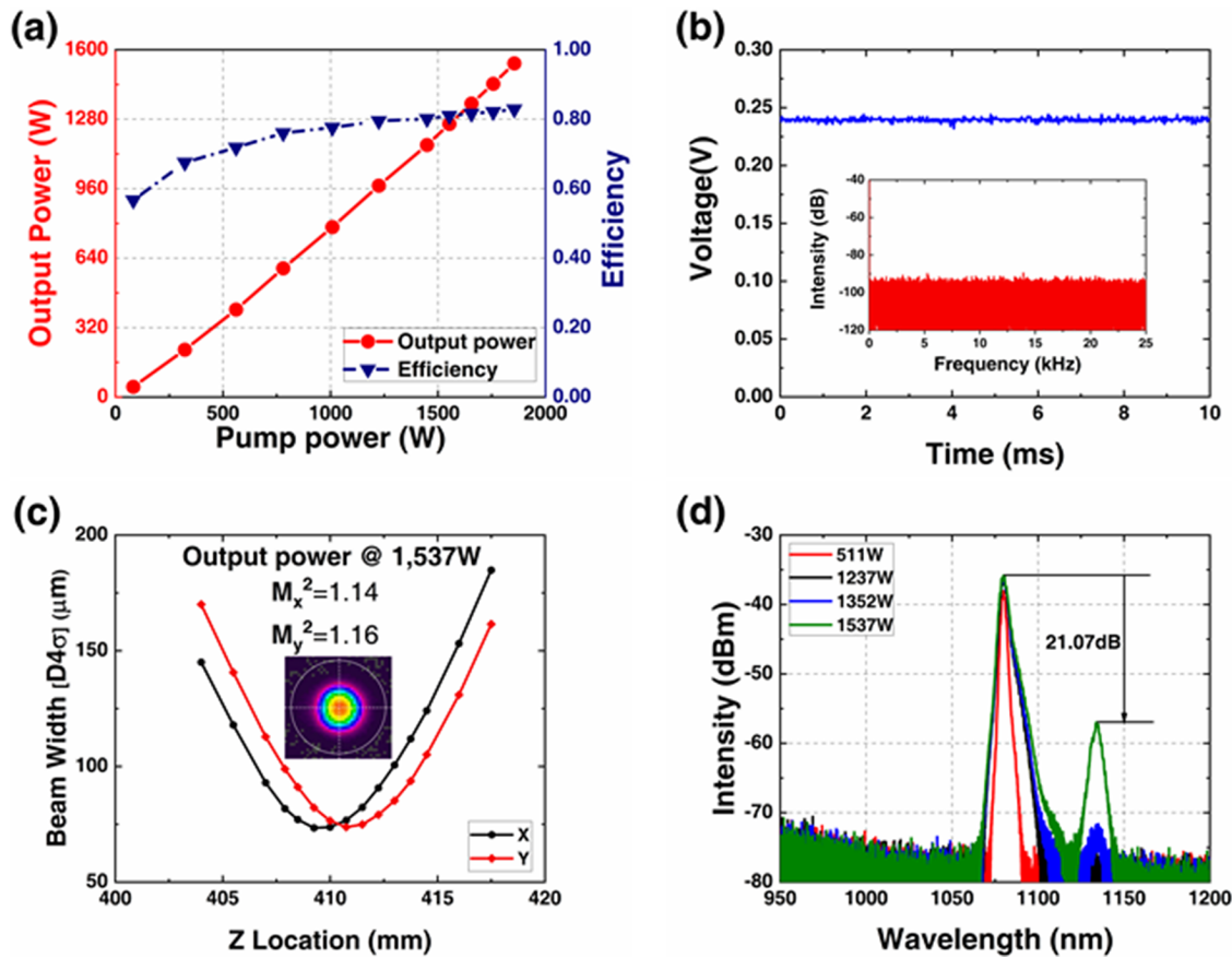
Figure 3. Experimental results of co-pumping: (a) variation curves of the output laser power and the O–O efficiency with the pump power; (b) signal of the PD at the maximum output power and their FFT results (inset); (c) result of the beam quality M^2 factor at the power of 1537 W (inset: the beam profile); (d) spectra at different output powers.
