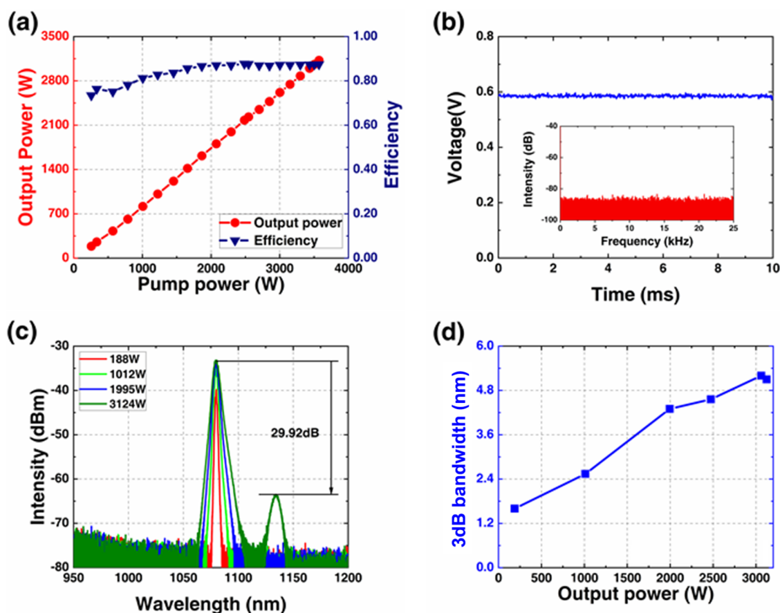
Figure 4. Experimental results of bidirectional pumping: (a) variation curves of the output laser power and the O–O efficiency with the pump power; (b) signal of the PD at the highest output power and their FFT results (inset); (c) spectra at different output powers; (d) measured 3-dB bandwidth at the different output powers.
