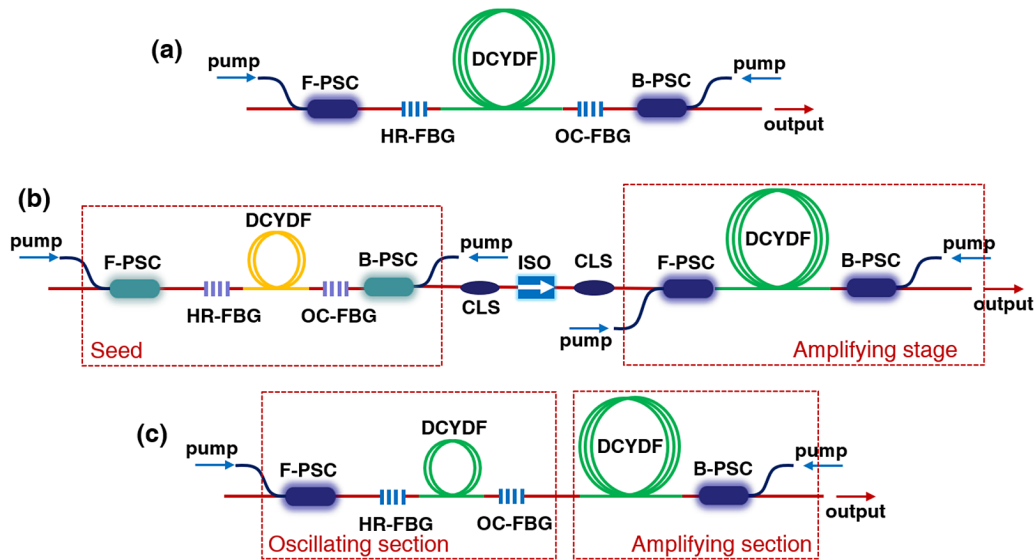
Figure 1. Schematic diagram of the three structures of fiber lasers: (a) fiber laser oscillator based on the FP-fiber cavity; (b) fiber laser amplifier based on the MOPA structure; (c) OAIFL.
