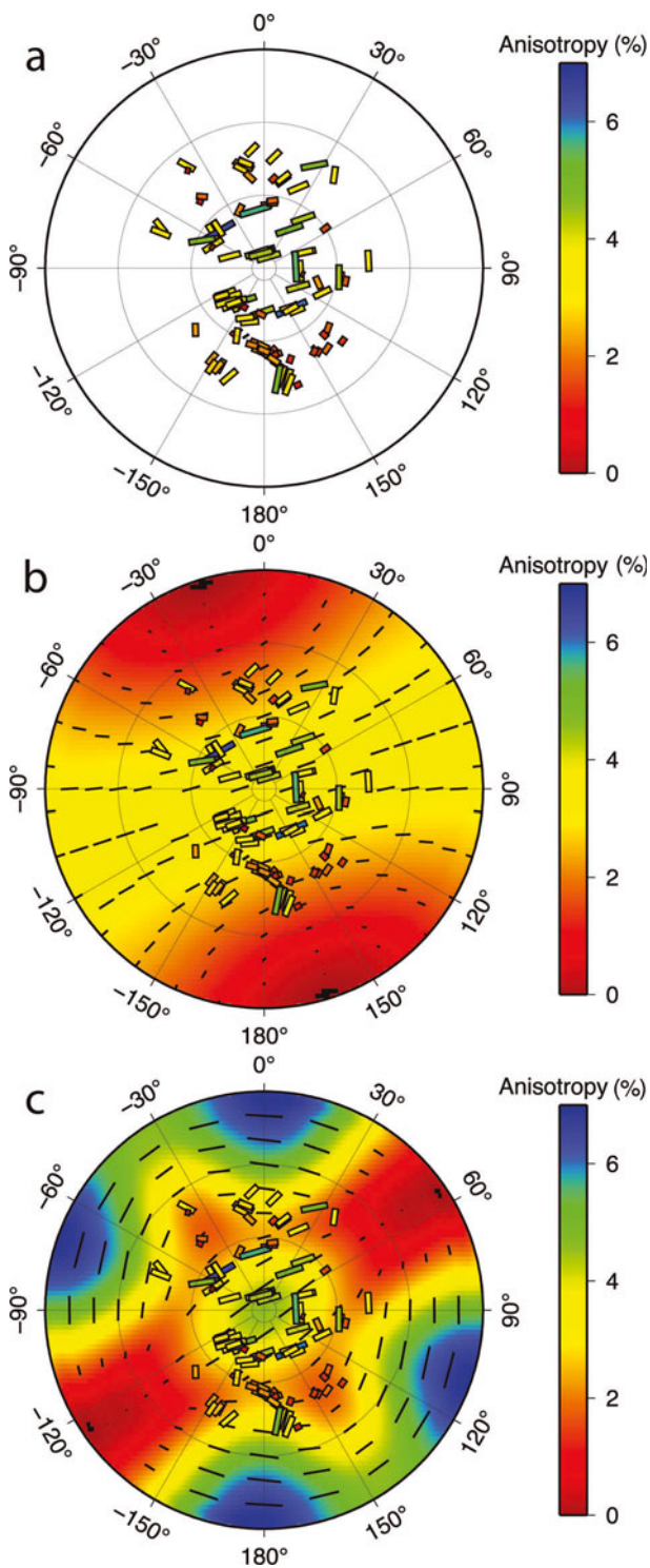
Fig. 8. (a) The shear-wave splitting results plotted on an upper-hemisphere projection. Vertical ray paths plot at the centre, and horizontally propagating rays would plot at the edge. The tick colour and length is proportional to the magnitude of the splitting, and its orientation shows the polarization of the fast shear wave. (b) Same as (a) but also showing the HTI model that best fits the shear-wave splitting measurements. This shows the orientation and magnitude of splitting for the girdle model that best explains the data. Black ticks show the orientation of the fast shear-wave polarization, and their length is proportional to the splitting. Colour scale indicates the magnitude of the anisotropy. (c) Same as (a) but also showing the orthorhombic model that best fits the shear-wave splitting measurements. The data are inverted for a model with vertically aligned cracks superimposed on a model with VTI symmetry. Black ticks show the orientation of the fast shear-wave polarization predicted by the model, and their length is proportional to the splitting. Ticks with a white outline are the fast shear-wave polarizations for the observations. Colour scale indicates the magnitude of the anisotropy.
