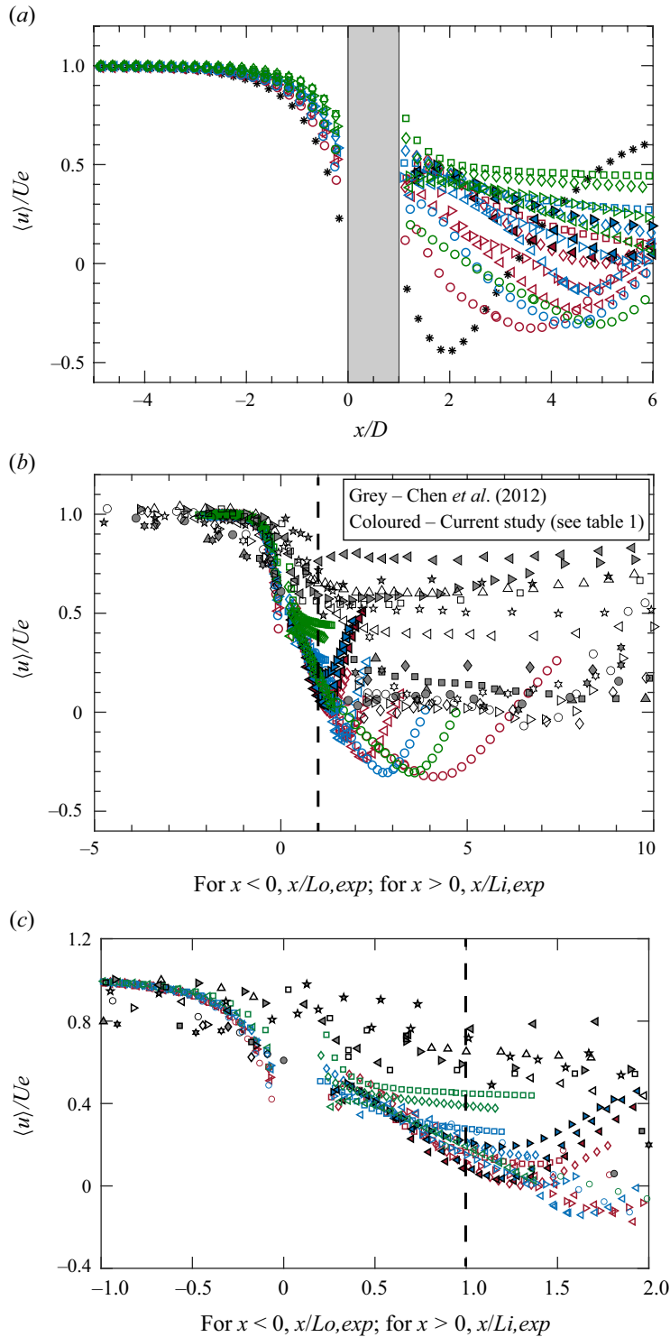
Figure 10. Longitudinal profiles of mean velocity ( \langle u \rangle / U_e ) along the centreline, (a) normalized by the cylinder width D , (b) normalized by the measured L_{i,exp} for x > 0 and L_{o,exp} for x < 0 and (c) normalized in the same manner as (b) but highlighting the collapsing trend near the porous cylinders. Symbols for the current study are summarized in table 1. Grey open and solid symbols are from figure 4 in Chen et al. (2012).
