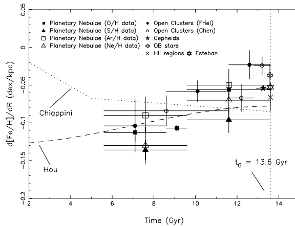
Figure 1. Time variation of the [Fe/H] gradient using PNe, open clusters, HII regions, Cepheids and OB stars. Theoretical models by Hou et al. (2000) and Chiappini et al. (2001) are also shown. The age of the galactic disk is taken as 13.6 Gyr.
