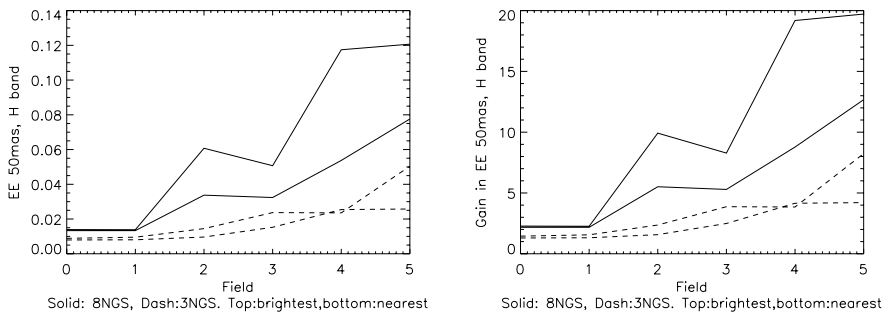
Figure 12. MOAO Ensquared Energy and Ensquared Energy gain relative to seeing for 1" seeing and several actual astronomical fields for the case of 50mas pixels and H band observations. Solid line: 8 NGSS, Dashed lines: 3 NGSS Top line: 8 (resp. 3) brightest NGSS, Bottom line: 8 (resp 3) nearest NGSS.
