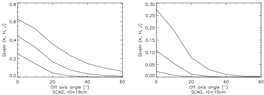
Figure 8. SCAO Strehl ratio loss due to anisoplanatism effect (top to bottom: K , H , J ). Left: 0.53'' Right: 1'' seeing.
