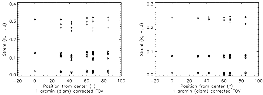
Figure 11. MCAO K, H, J band Strehls (top to bottom) versus FoV position for a constellation of 6 NGSS (3 in a 2' FoV and 3 in a 6' FoV) with 0.53" seeing. Left: 5th magnitude NGSS, Right: 17th magnitude NGSS.
