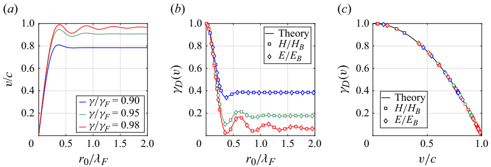
Figure 3. The dependence of energy on the steady orbital speed, v , computed using (4.3) for \gamma/\gamma_F taking values 0.9 (blue), 0.95 (green) and 0.98 (red). (a) The orbital speed oscillates over half the Faraday wavelength as the orbital radius, r_0 , is increased, approaching the rectilinear walking speed, v_0 , for large radii. The variations in the orbital speed are most pronounced close to the Faraday threshold. (b, c) The magnitude of the local wave height, H (squares), and stroboscopic wave energy, E (diamonds), relative to that of a bouncer ( H_B and E_B , respectively) as a function of (b) orbital radius, r_0 , and (c) orbital speed, v . The numerical results coincide with the theoretical predictions H/H_B = \gamma_D(v) and E/E_B = \gamma_D(v) for steady droplet motion (see § 3) indicated by the black curve, where \gamma_D(v) = 1 - v^2/c^2 is the speed-dependent diminution factor (see (2.4)). The physical parameter values are the same as in figure 1.
