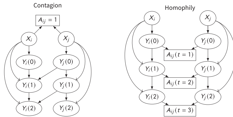
Figure 1. DAGs for the contagion versus homophily-only data generation models used for the simulation data.
